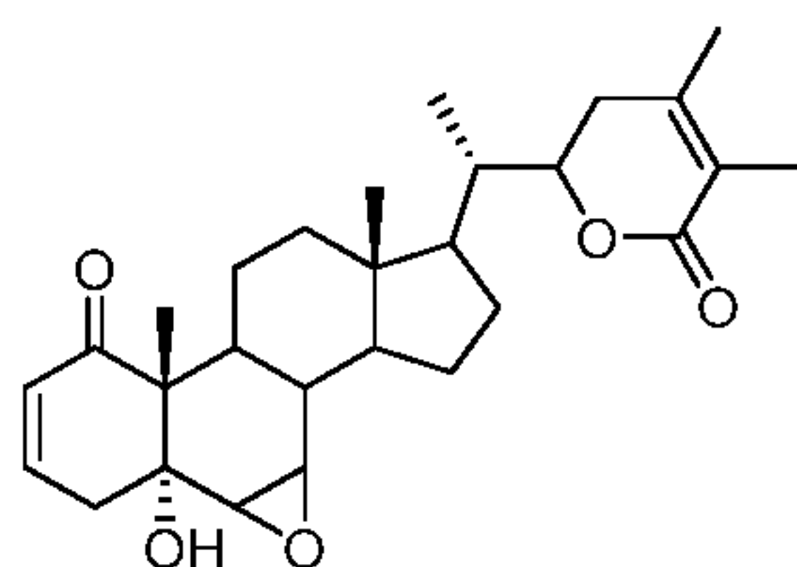
Withanolide B
