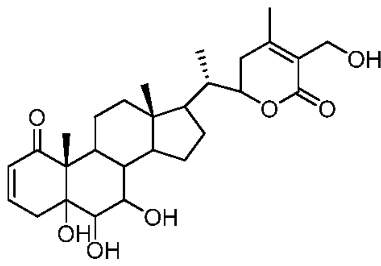
Withanolide LN
