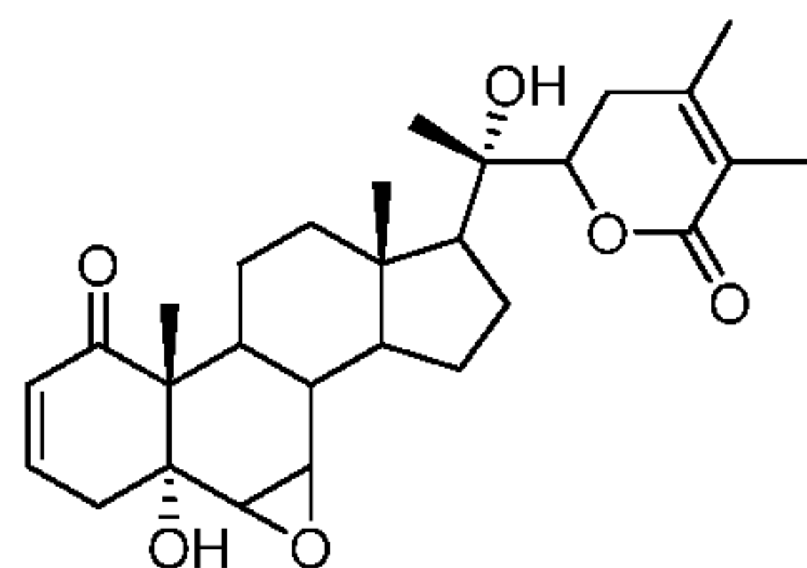
Withanolide A
