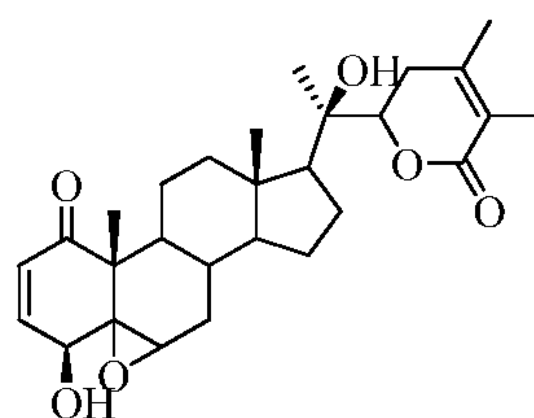
Withanolide D
