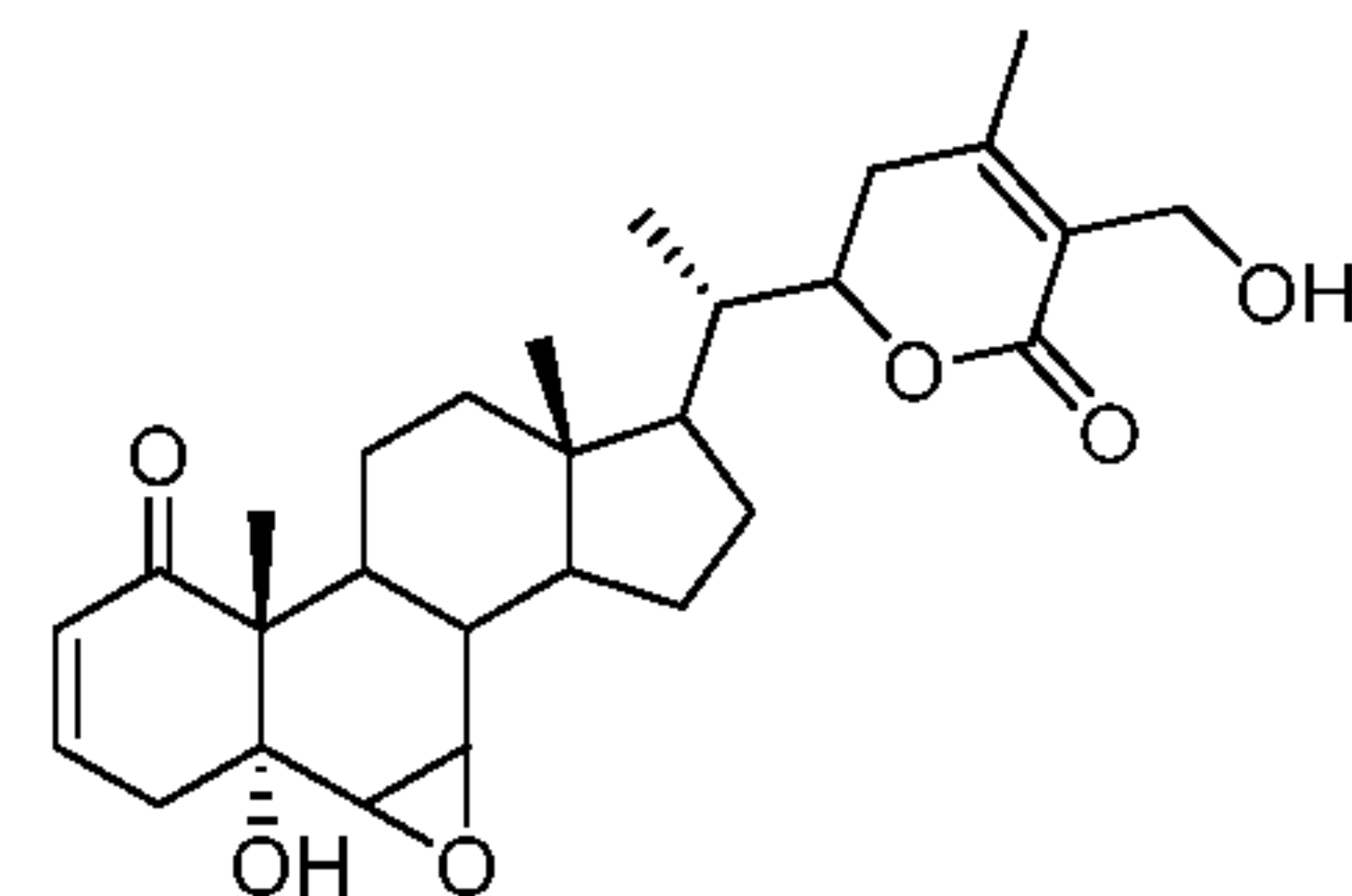
12-deoxy withastramonolide
