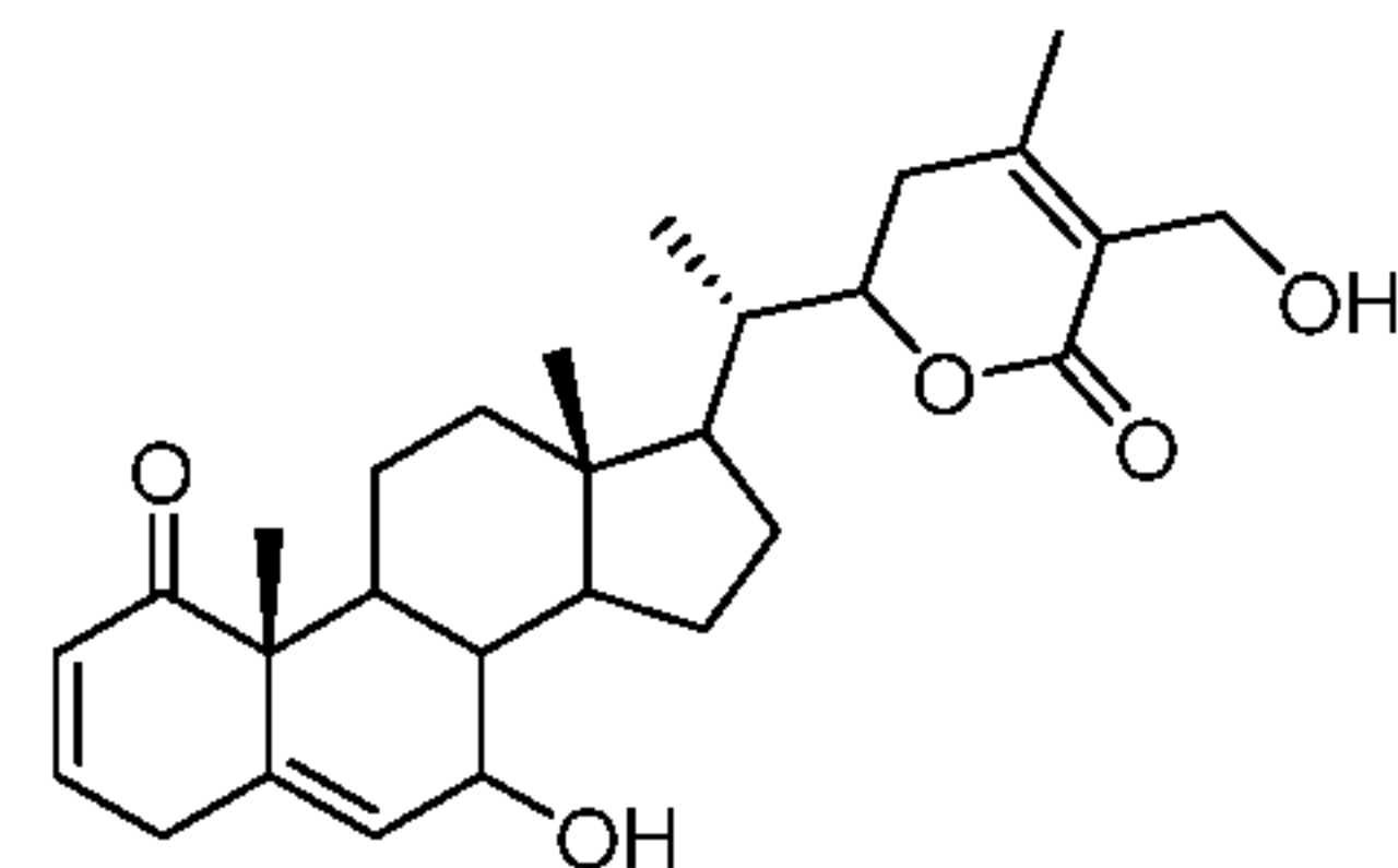
7,27-dihydroxy-1-oxo-witha-2,5,24-trienolide
