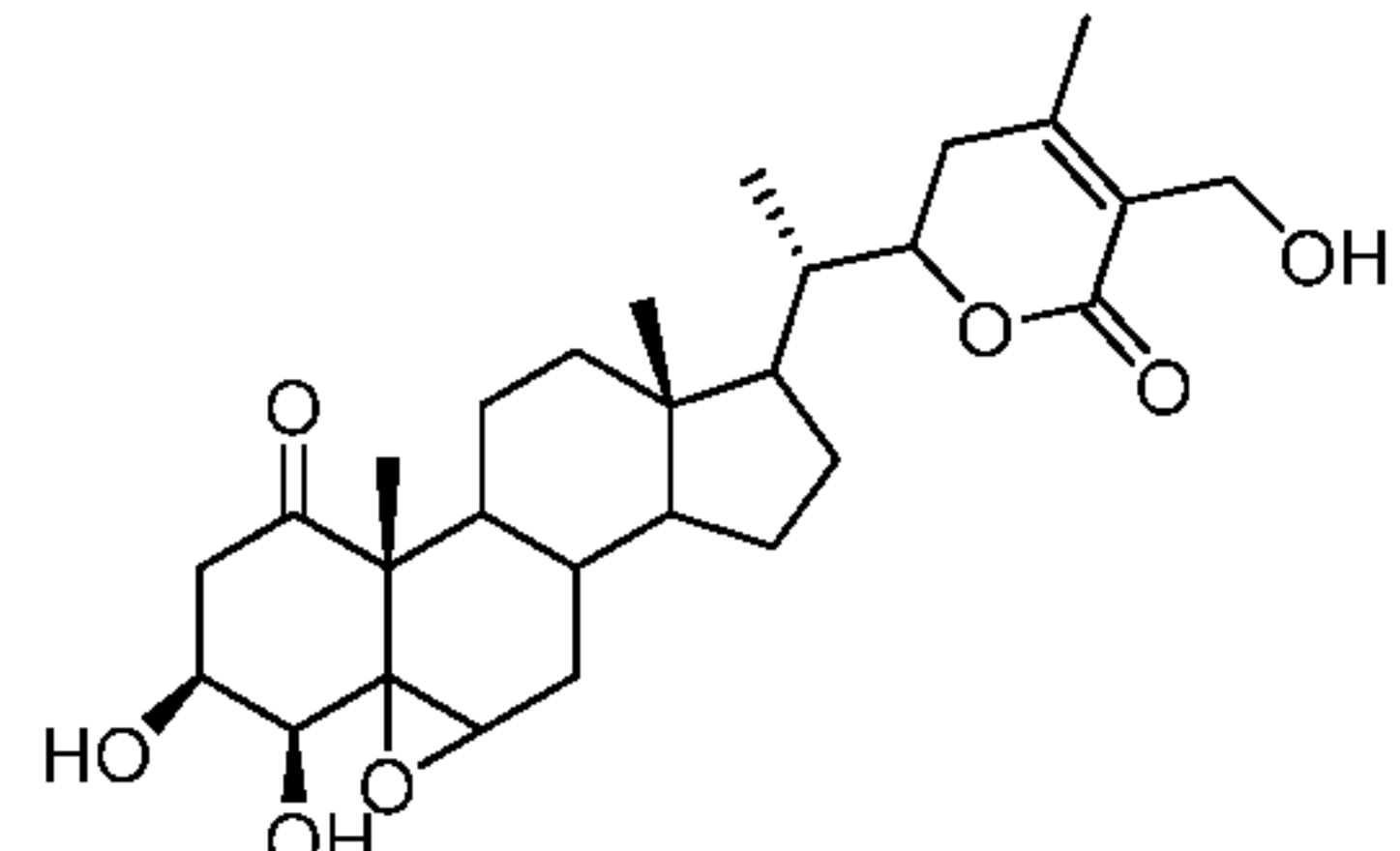
3-Hydroxy withferin-A
