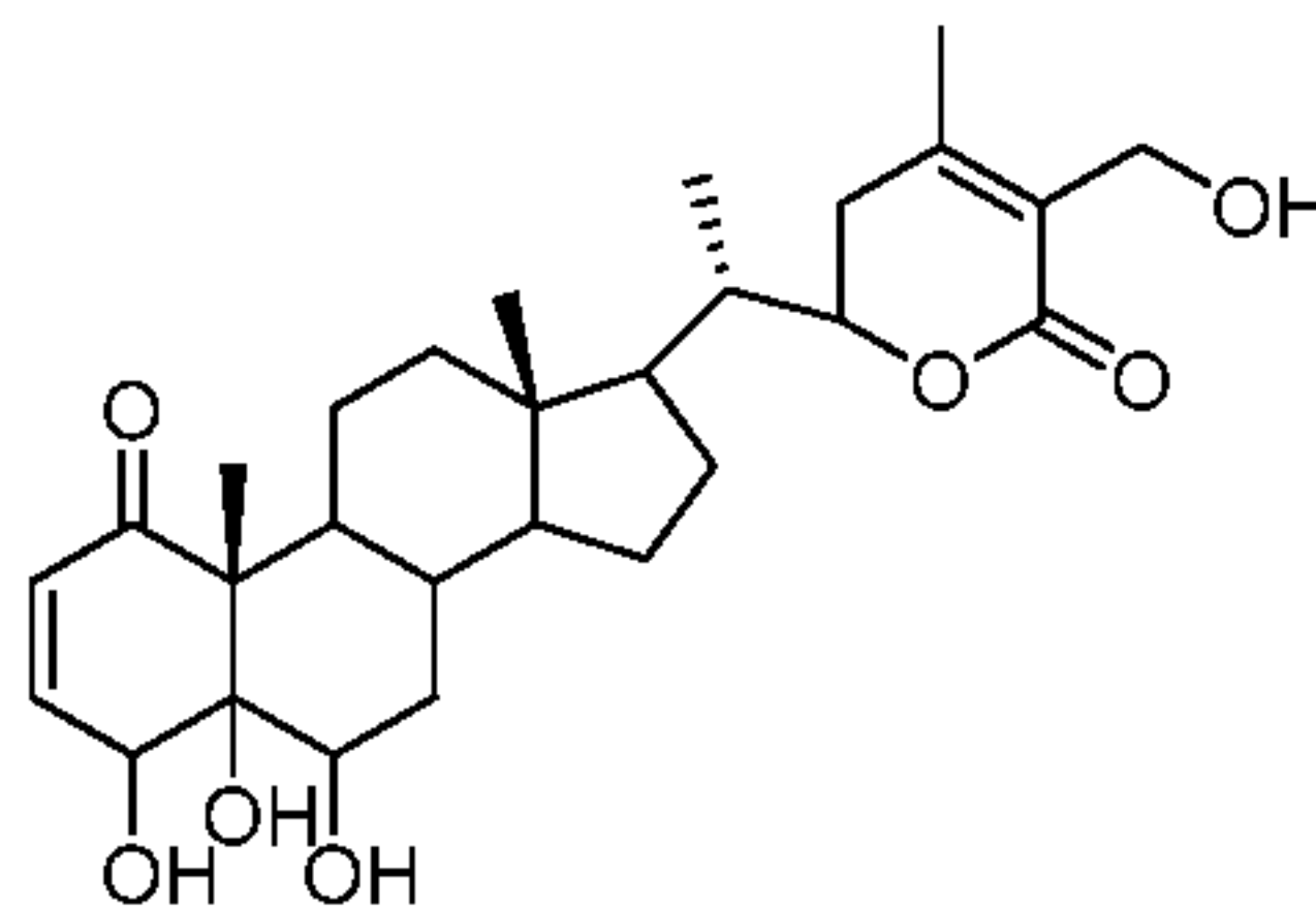
2,3-dehydrosomnifericin
