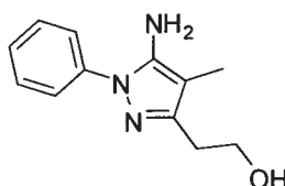
2-(5-amino-4-methyl-1-phenyl-1H-pyrazol-3-yl)ethanol
