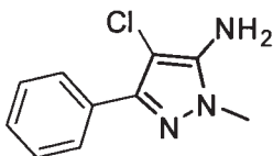
4-chloro-1-methyl-3-phenyl-1H-pyrazol-5-amine
