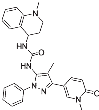
1-(1-methyl-1,2,3,4-tetrahydroquinolin-4-yl)-3-(4-methyl-3-(1-methyl-6-oxo-1,6-dihydropyridin-3-yl)-1-phenyl-1H-pyrazol-5-yl)urea
