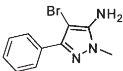
4-bromo-1-methyl-3-phenyl-1H-pyrazol-5-amine
