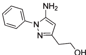
2-(5-amino-1-phenyl-1H-pyrazol-3-yl)ethanol
