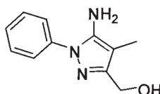
(5-amino-4-methyl-1-phenyl-1H-pyrazol-3-yl)methanol
