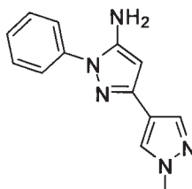
1'-methyl-1-phenyl-1H,1'H-3,4'-bipyrazol-5-amine
