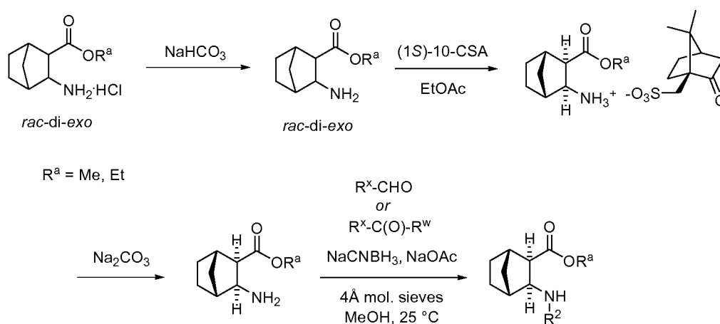
Scheme 7
