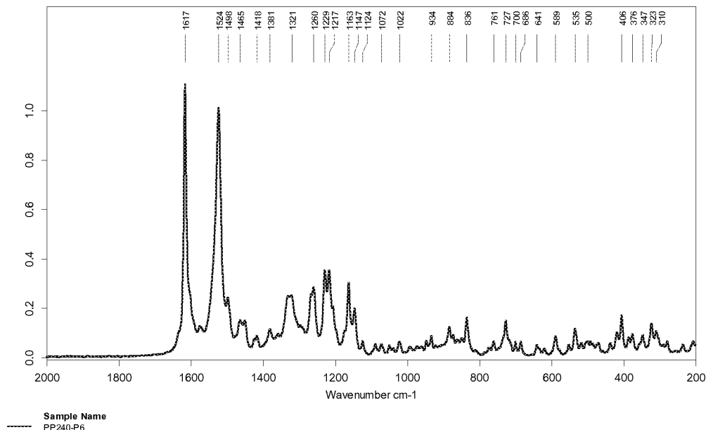
Graph 2. FT-Raman Spectrum.
