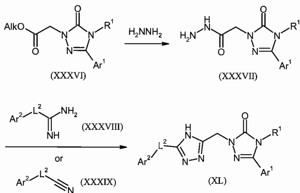
Scheme 8
