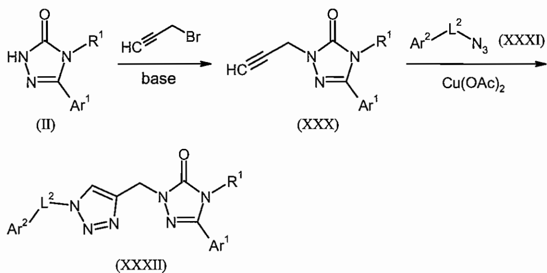
Scheme 6
