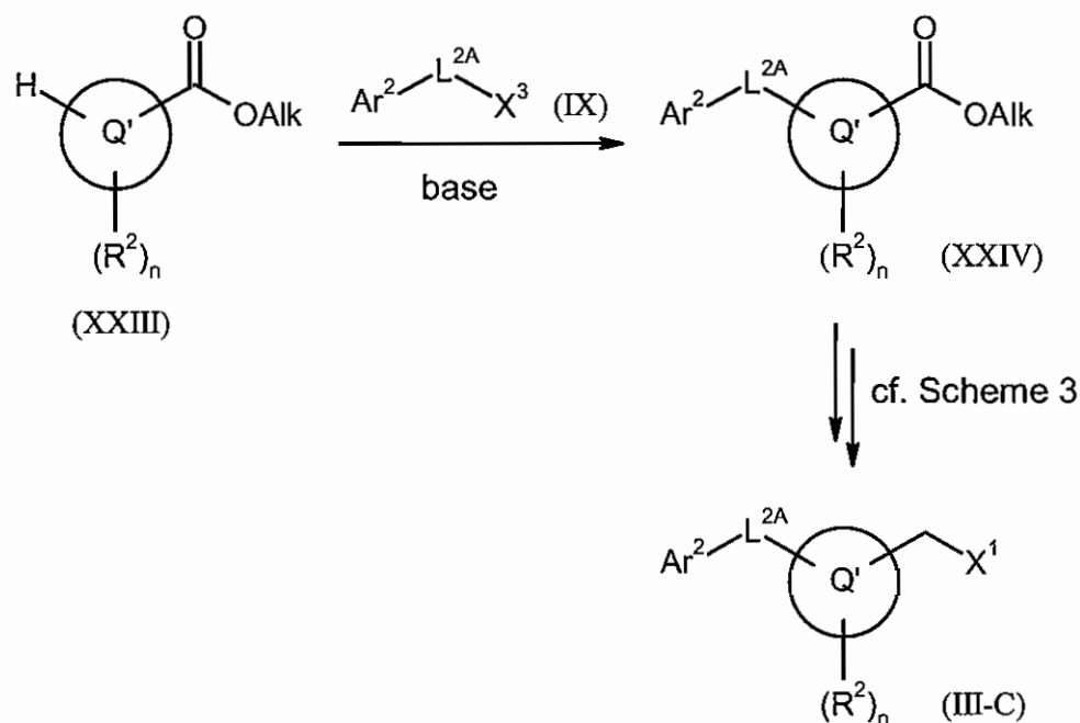
Scheme 4
