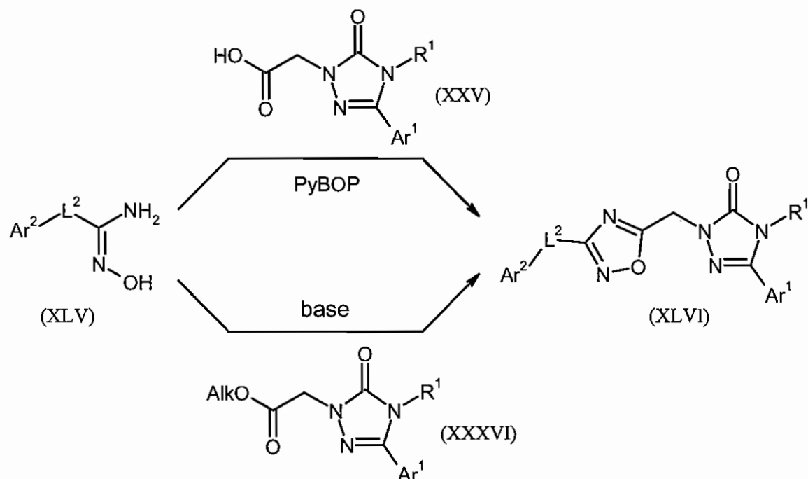
Scheme 10
