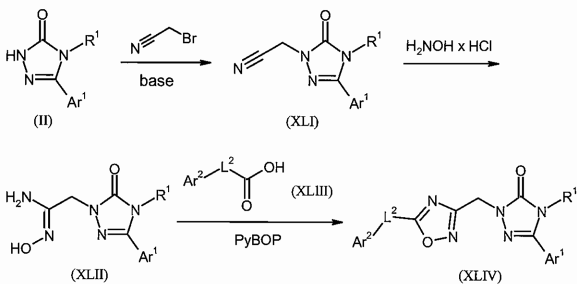
Scheme 9
