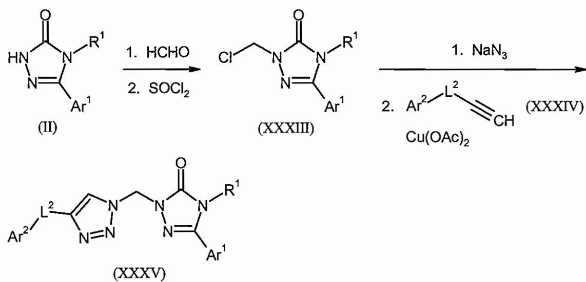
Scheme 7
