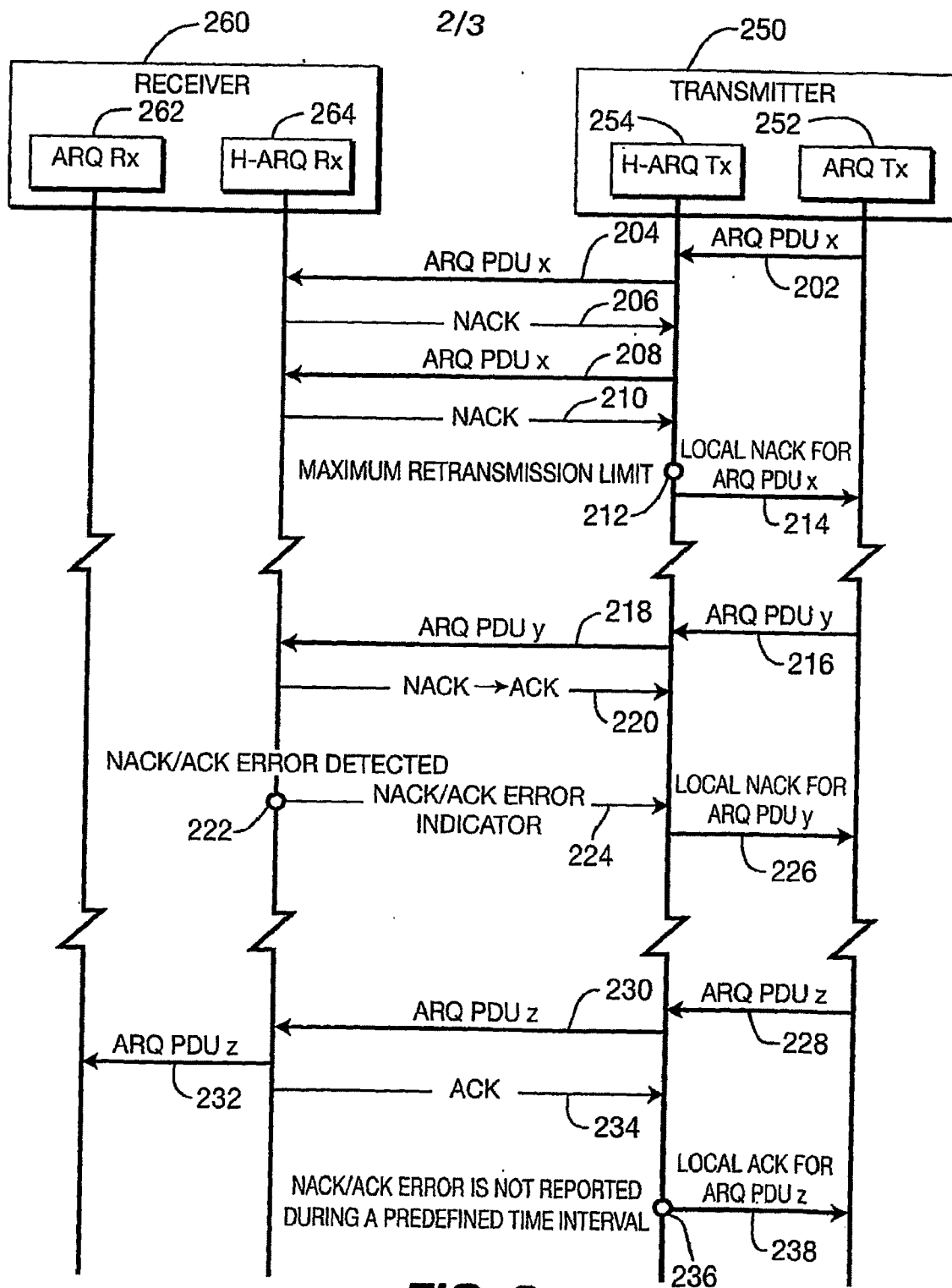
FIG. 2 PRIOR ART
