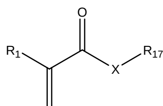
FORMULA IX
