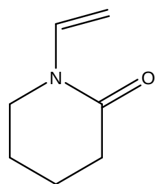
Formula V
