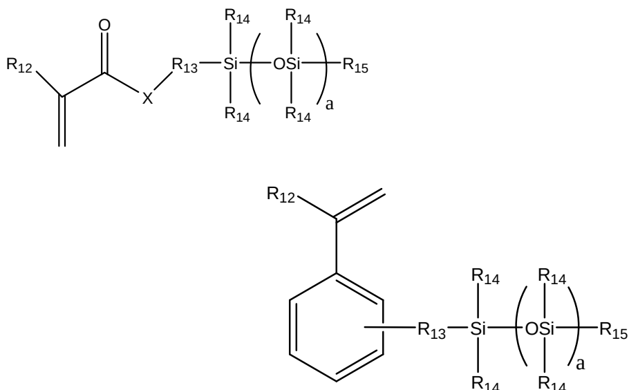
Formula VIII
