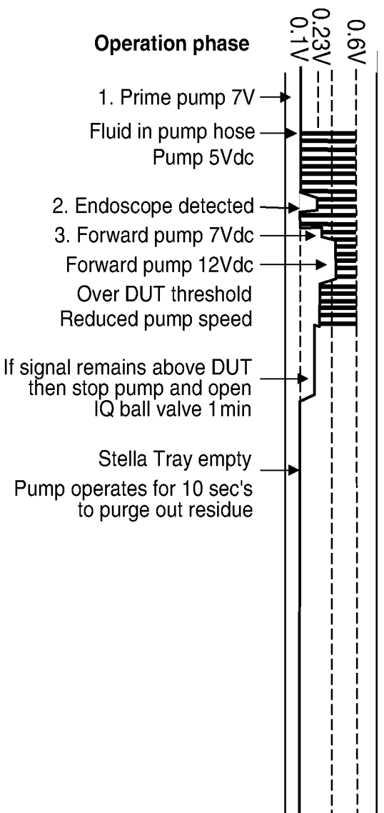
Start of disinfection clean cycle and endoscope with a small diameter Luer channel
