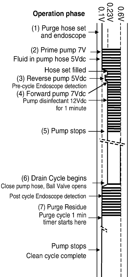
Typical waveform for 5 minute disinfection clean cycle with endoscope detection
