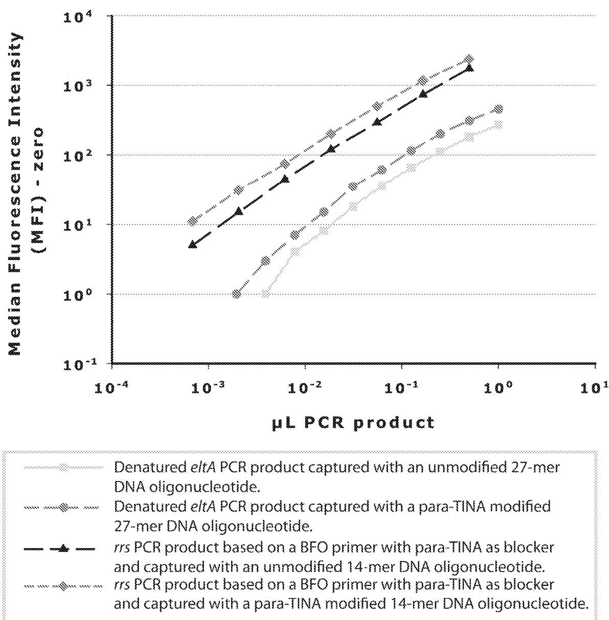
Figure 1: Detection of denatured PCR product versus BFO modified PCR product
