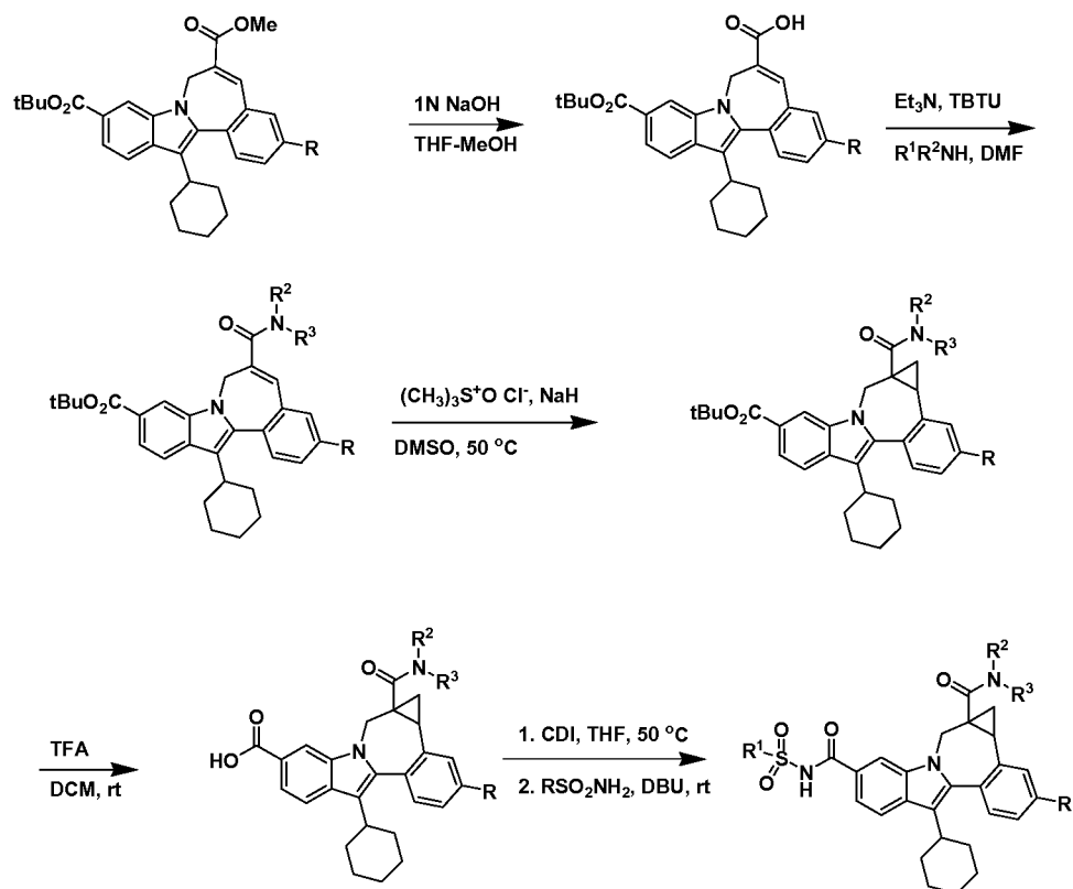
Scheme 4a.
