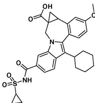
Intermediate 30
