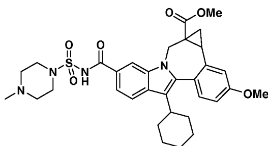
Intermediate 38
