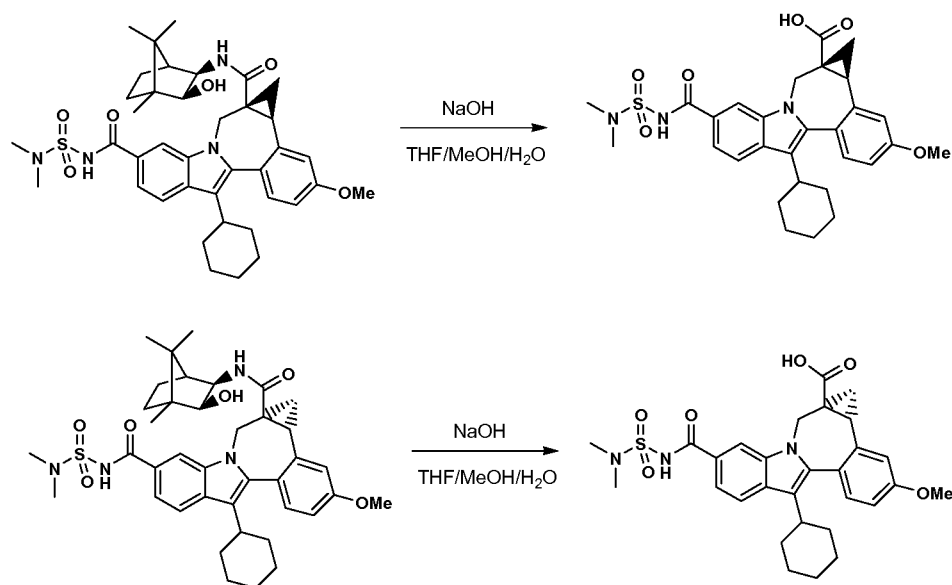
Scheme 7.
