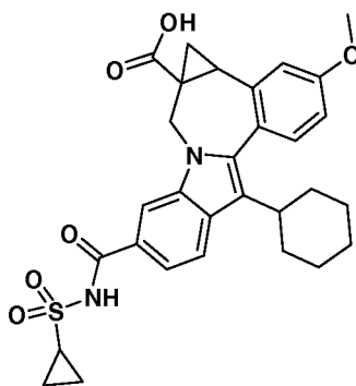
Intermediate 27
