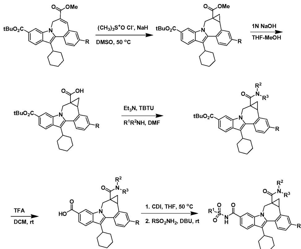
Scheme 4b.
