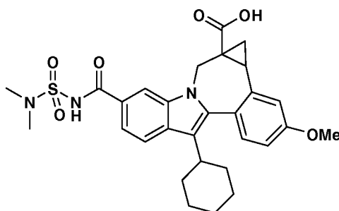
Intermediate 10
