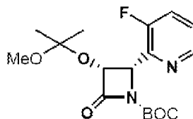
formula (VI)
