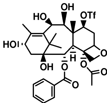
formula (X).
