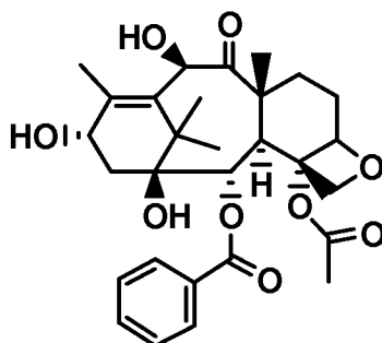
formula (XI).
