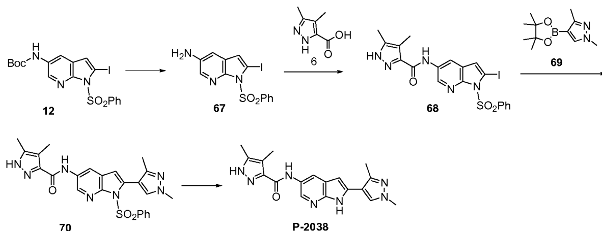
Scheme 12
