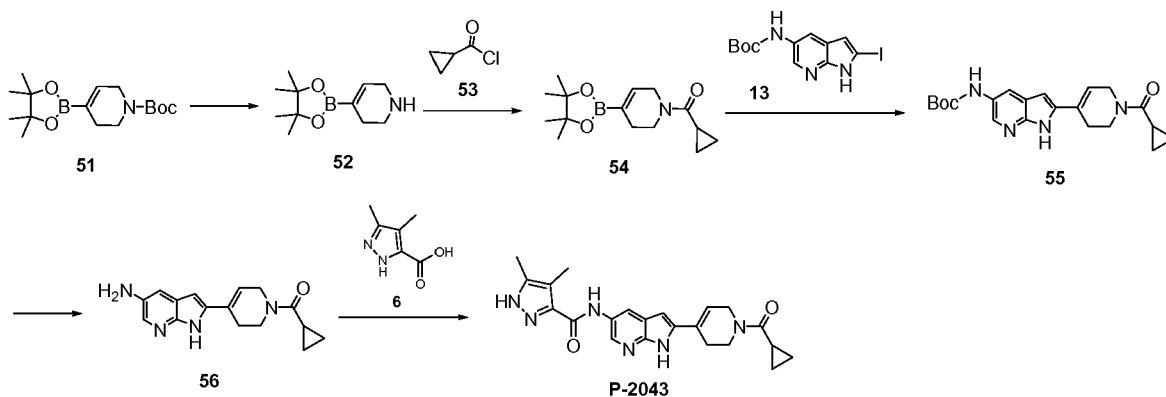
Scheme 9.
