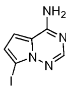
Formula (VII)
