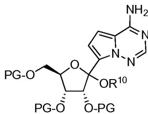
Formula (V)
