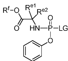
Formula (X),
