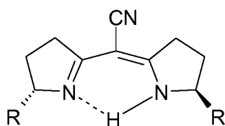
Semicorrin
