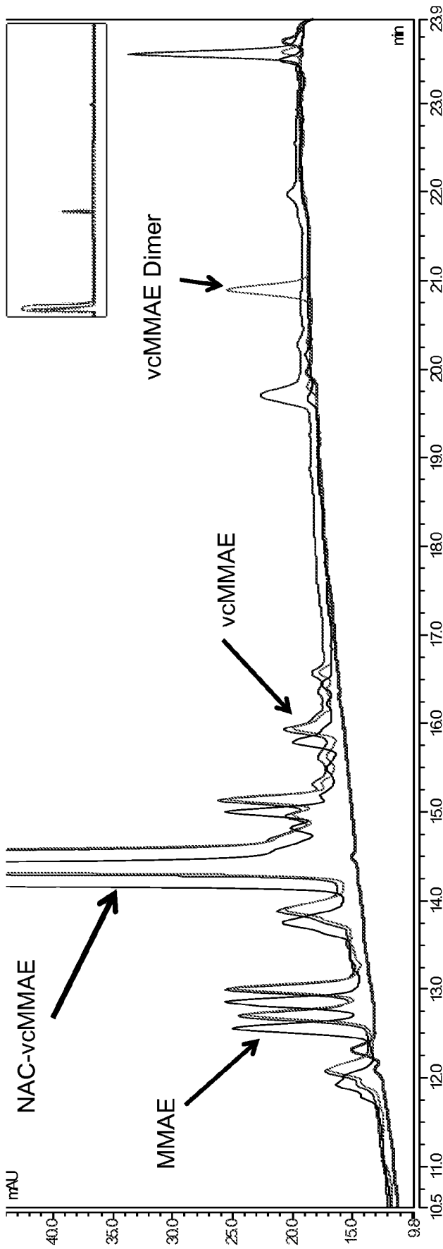
aMUC16-vcMMAE- Reduction with TCEP Legend: Sparged with Nitrogen 5min. Sparged with Air 5min. No Sparge- Control aMUC16 Unconjugated Bulk Intermediate
