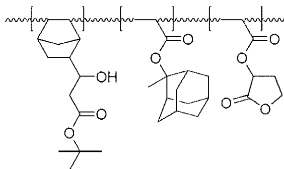
[Chemical Formula 10]
