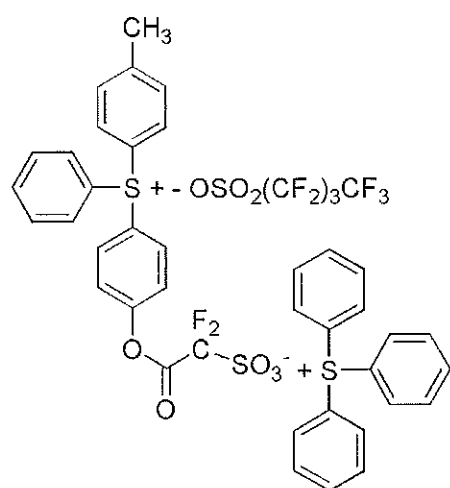
[Chemical Formula 6-10]
