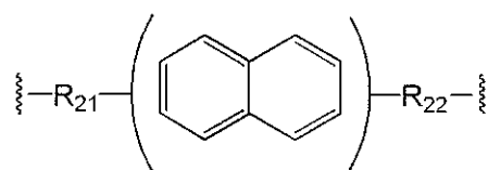
[Chemical Formula 2-3]
