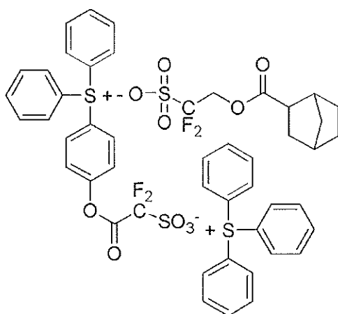
[Chemical Formula 6-5]
