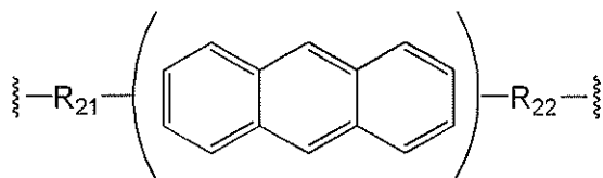
[Chemical Formula 2-4]
