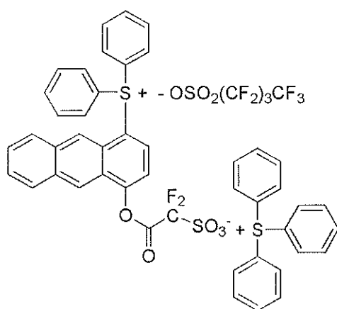
[Chemical Formula 6-15]
