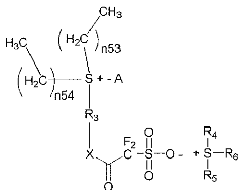
[Chemical Formula 5-3]
