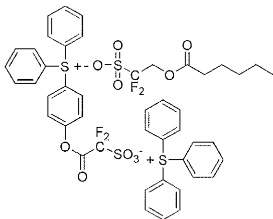
[Chemical Formula 6-7]
