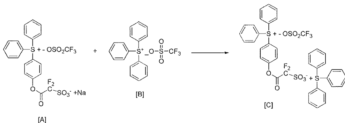
(Synthesis Example 2)
