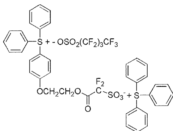
[Chemical Formula 6-9]
