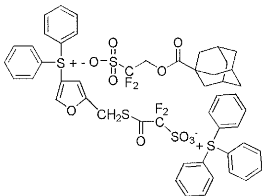
[Chemical Formula 6-22]
