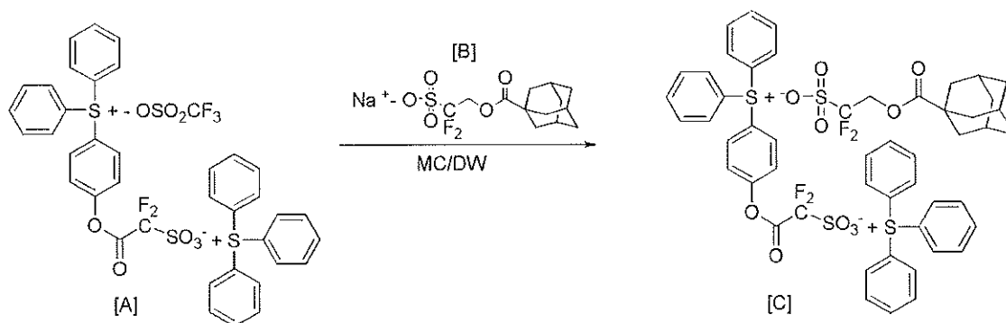
[Reaction Scheme 3]
