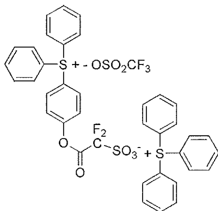
[Chemical Formula 6-2]
