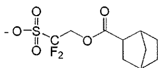
[Chemical Formula 1-7]
