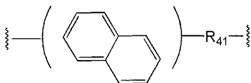
[Chemical Formula 4-3]
