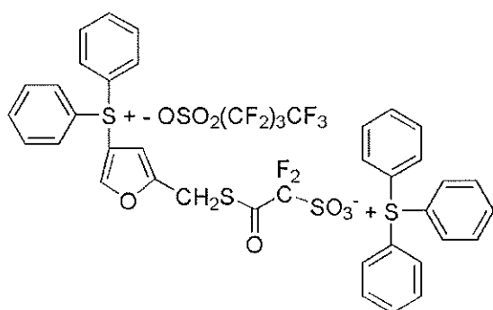
[Chemical Formula 6-21]
