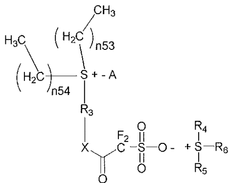
[Chemical Formula 5-3]
