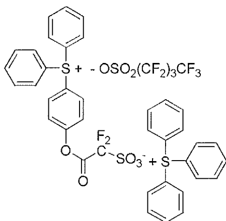
[Chemical Formula 6-3]
