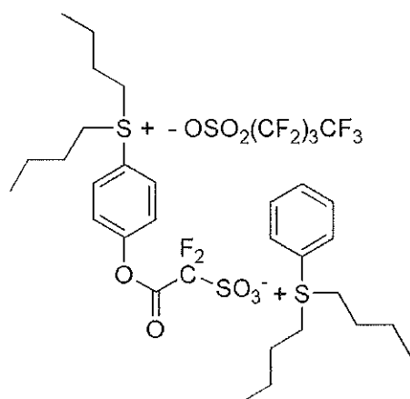
[Chemical Formula 6-17]
