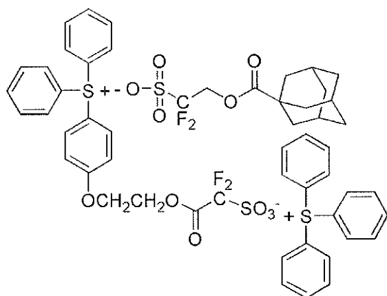
[Chemical Formula 6-10]
