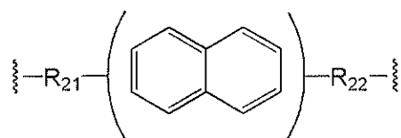
[Chemical Formula 2-3]
