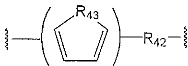
[Chemical Formula 4-4]
