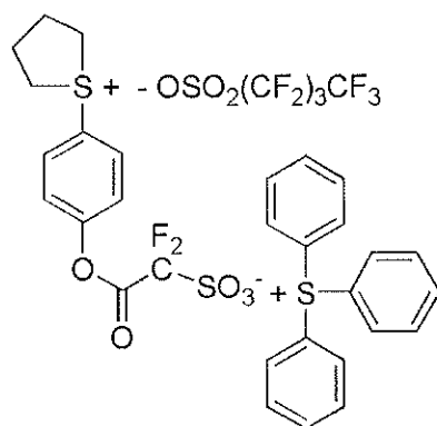
[Chemical Formula 6-17]
