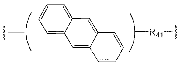
[Chemical Formula 4-4]
