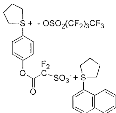
[Chemical Formula 6-19]
