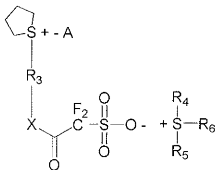
[Chemical Formula 5-3]
