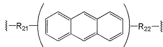
[Chemical Formula 2-4]
