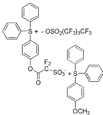
[Chemical Formula 6-12]
