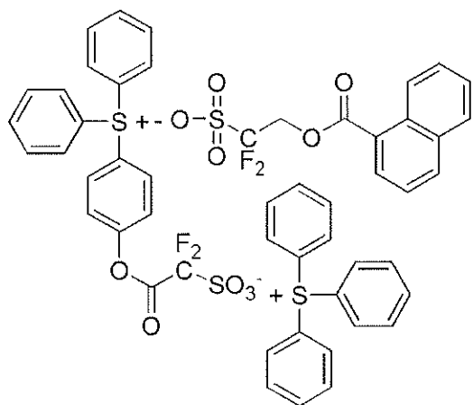
[Chemical Formula 6-6]
