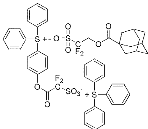
[Chemical Formula 6-4]
