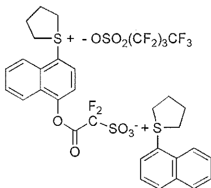
[Chemical Formula 6-20]
