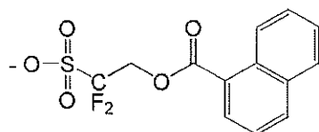
[Chemical Formula 1-8]
