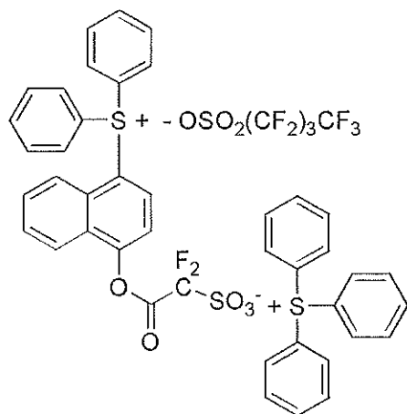
[Chemical Formula 6-14]
