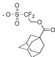
[Chemical Formula 1-6]
