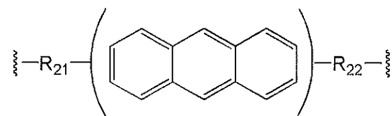
[Chemical Formula 2-4]
