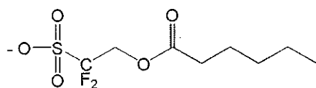
[Chemical Formula 1-8]
