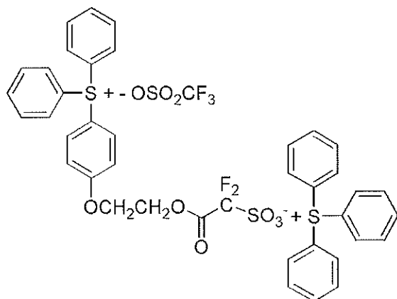
[Chemical Formula 6-8]
