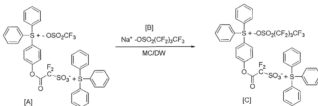
[Reaction Scheme 2]
