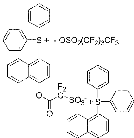
[Chemical Formula 6-16]
