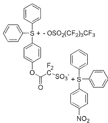
[Chemical Formula 6-13]
