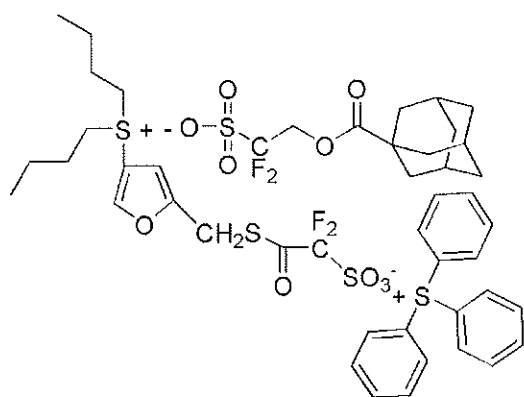
[Chemical Formula 6-22]
