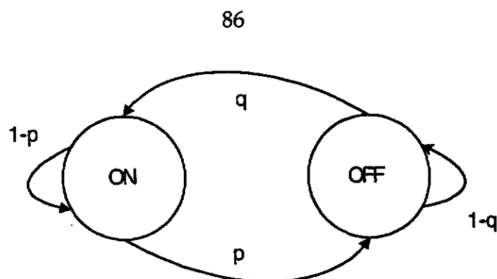
Figure 3. Two-state Markov chain representing ON/OFF transitions for TDSO
