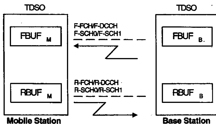
Figure 1. Synchronized operation of pseudo-random number generated buffers
