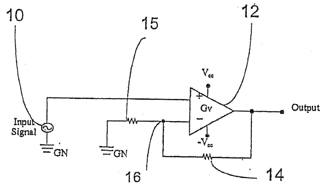
Fig. 1 Conventional Amplifier, Typically Class B
