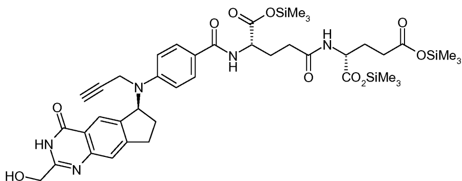
( R )-bis(trimethylsilyl) 2-(( S )-4-(4-((( S )-2-(hydroxymethyl)-4-oxo-4,6,7,8-tetrahydro-3 H -cyclopenta[ g ]quinazolin-6-yl)- N -(prop-2-ynyl)amino)benzamido)-5-oxo-5-(trimethylsilyloxy)pentanamido)pentanedioate;
