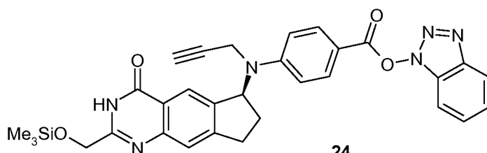
( S )-1 H -Benzo[ d ][1,2,3]triazol-1-yl 4-((2-(trimethylsiloxymethyl)-4-oxo-4,6,7,8-tetrahydro-3 H -cyclopenta[ g ]quinazolin-6-yl)- N -(prop-2-ynyl)amino)benzoate 24 ;
