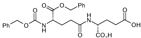
( R )-2-(( S )-5-(benzyloxy)-4-(benzyloxycarbonylamino)-5-oxopentanamido)pentanedioic acid;
