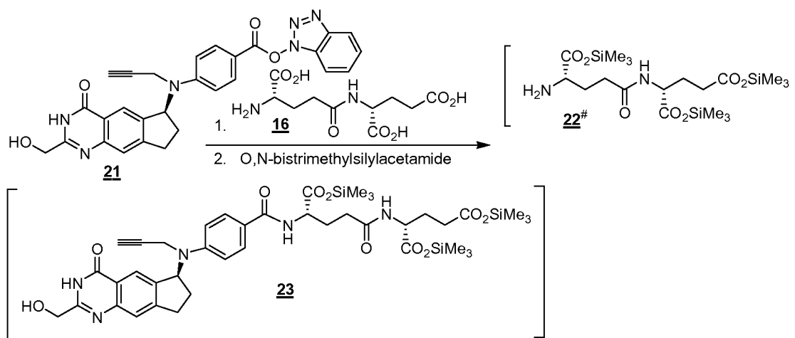
Scheme 4b. # This intermediate may also be trimethylsilylated
