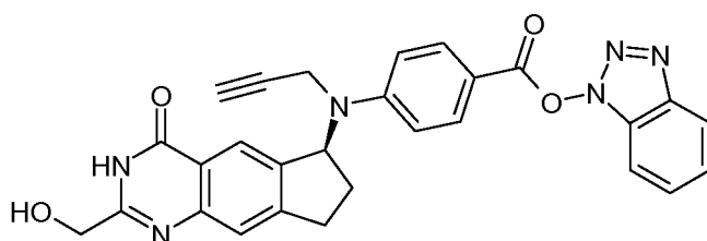
( S )-1 H -benzo[ d ][1,2,3]triazol-1-yl 4, N -((2-(hydroxymethyl)-4-oxo-4,6,7,8-tetrahydro-3 H -cyclopenta[ g ]quinazolin-6-yl)- N -(prop-2-ynyl)amino)benzoate;
