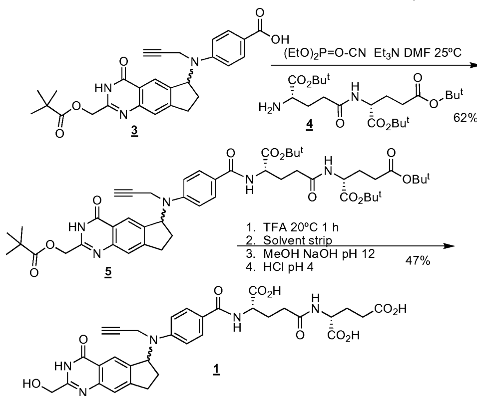
Scheme 1. Original Synthesis of Compound 1 as a pair of 6-Diastereoisomers
