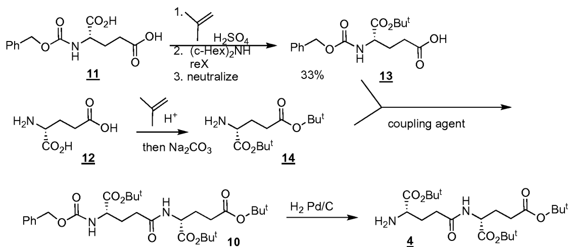
Scheme 3. Shortest synthesis of tri- O - t -butyl L-glutamyl- \gamma -D-glutamate, 4 .
