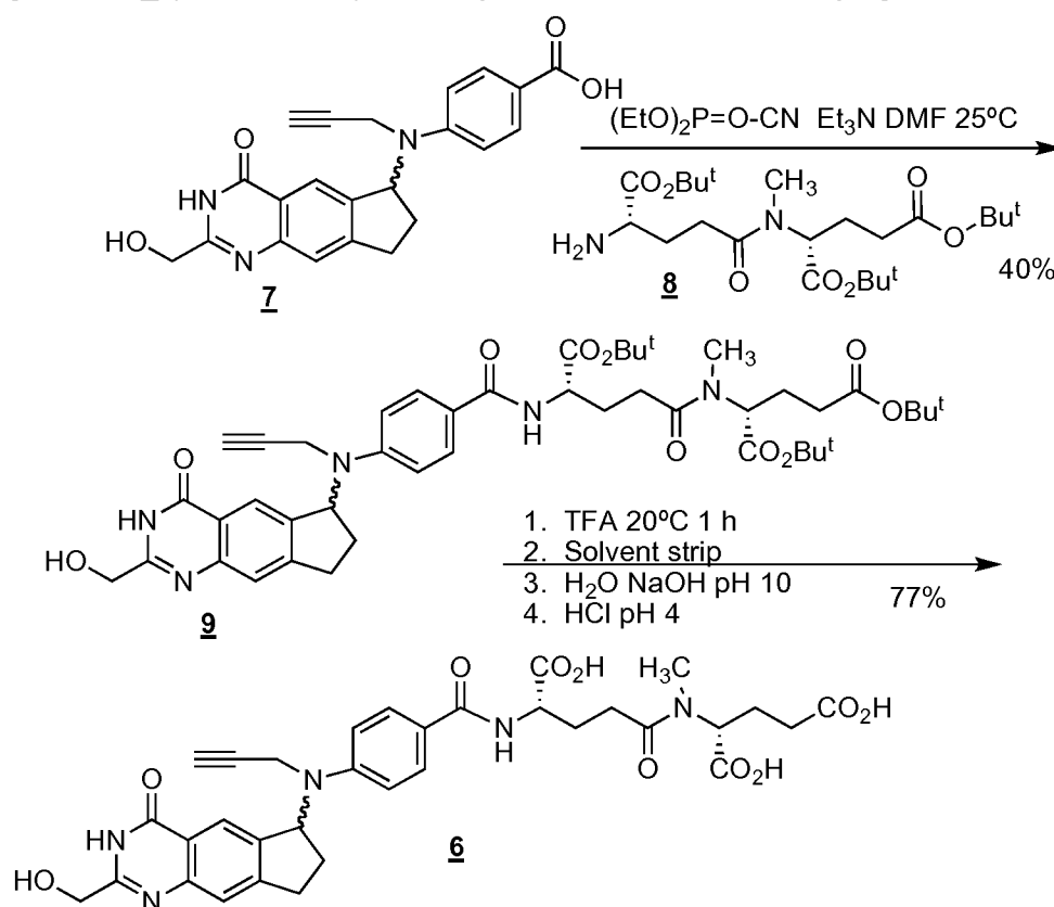
Scheme 2. Synthesis of N -Methyl Analogue of Acid 1 from Hydroxyacid 7 .
