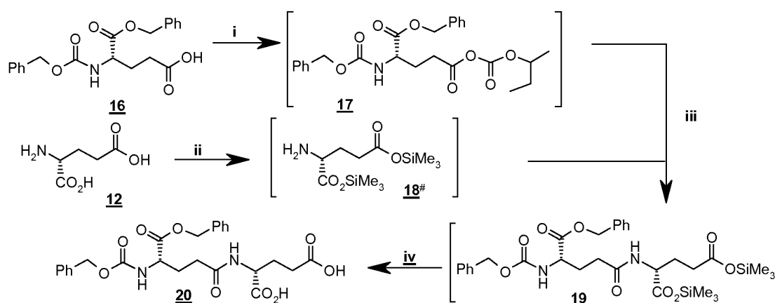
Scheme 4a. (i) NMM IBCF THF -30 °C (ii) BSA THF 20 °C (iii) Add 18 to 17 -30 to 20 °C (iv) EtOAc water pH2 reX ACN # This intermediate may also be N-trimethylsilylated
