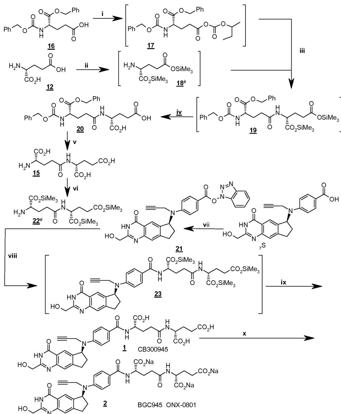
Scheme 4. Process of the invention for an efficient synthesis of Compound 2
