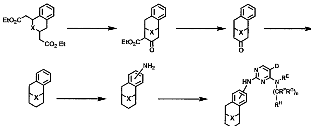
Scheme 11
