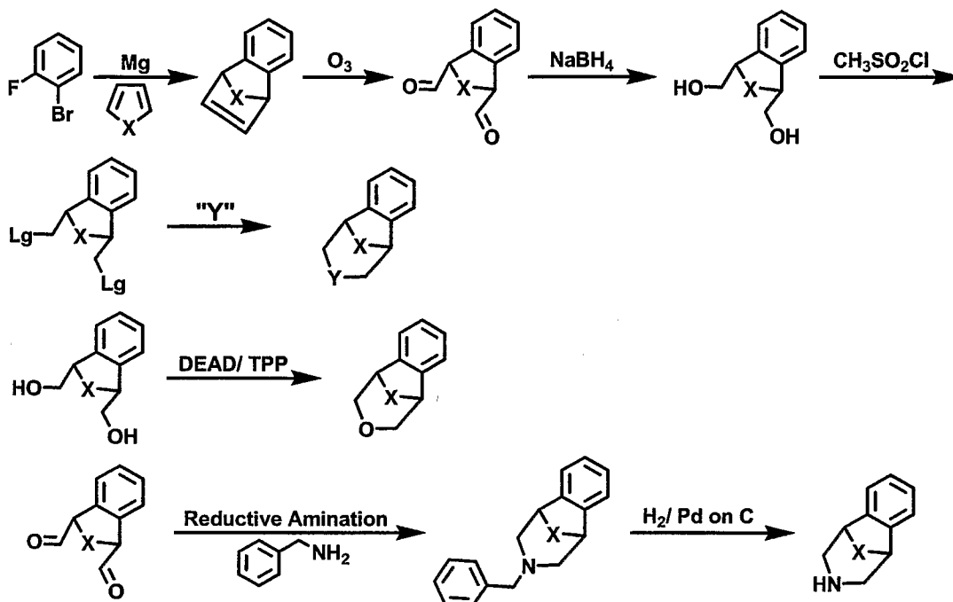
Scheme 8
