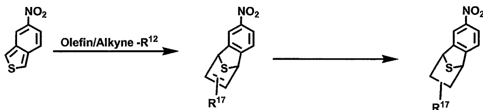
Scheme 7b
