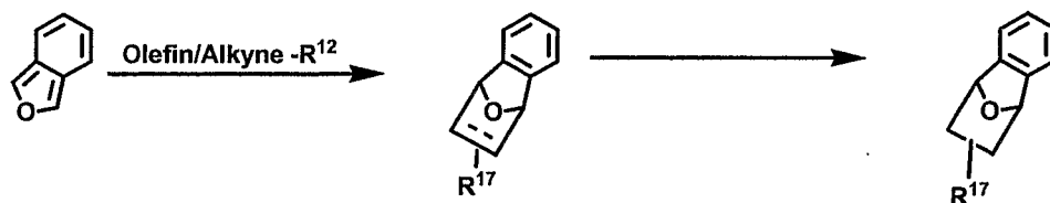
Scheme 7b
