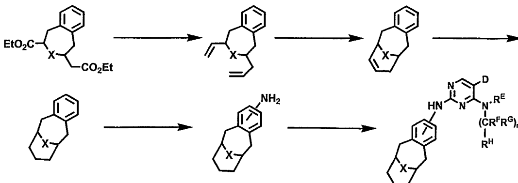
Scheme 12
