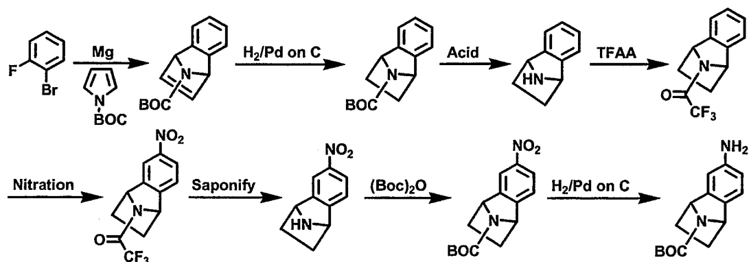
Scheme 4
