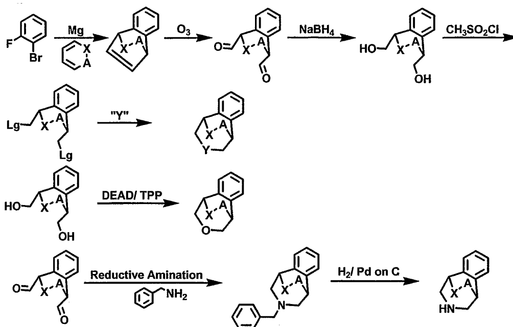
Scheme 9
