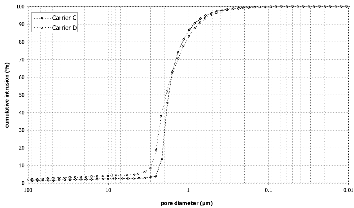
FIGURE 6 Cumulative Intrusion vs Pore size
