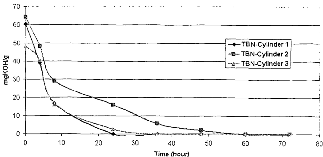
Bolnes Engine Test - TBN Analyses of the Drain Oils
