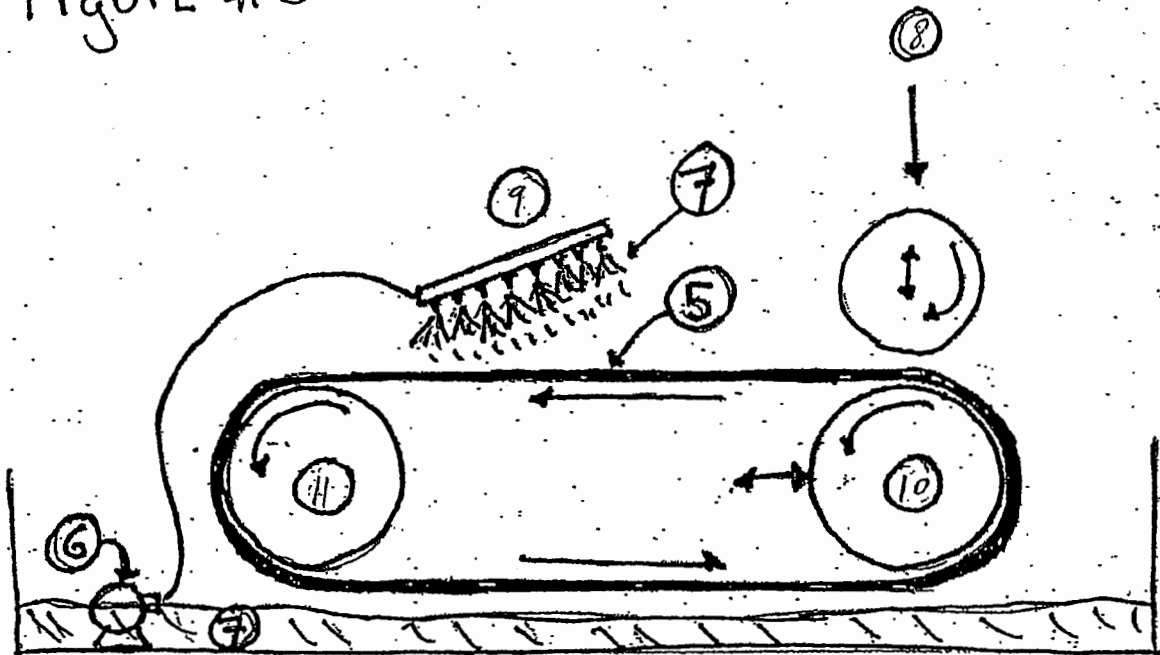
Figure 5. Simulated Belt Polish Apparatus
