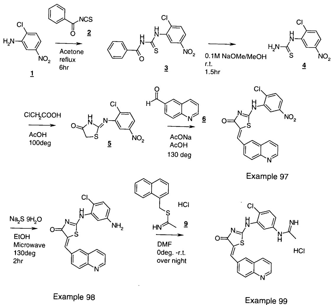
Scheme D
