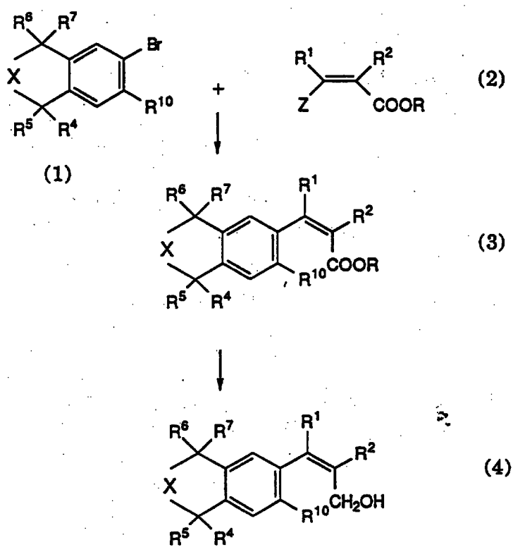
Scheme 1
