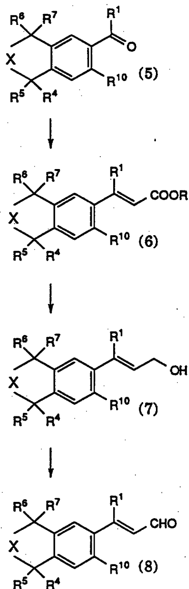
Scheme 2
