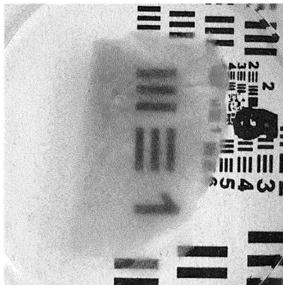
Methyl salicylate - benzyl benzoate
