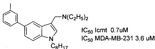
N-ethyl-N-[(1-octyl-5-m-tolyl-1H-indol-3-yl)methyl]ethanamine
