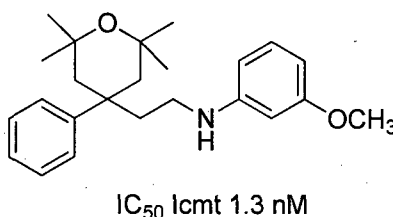
3-methoxy-N-[2-(2,2,6,6-tetramethyl-4-phenyltetrahydro pyran -4-yl)ethyl]aniline
