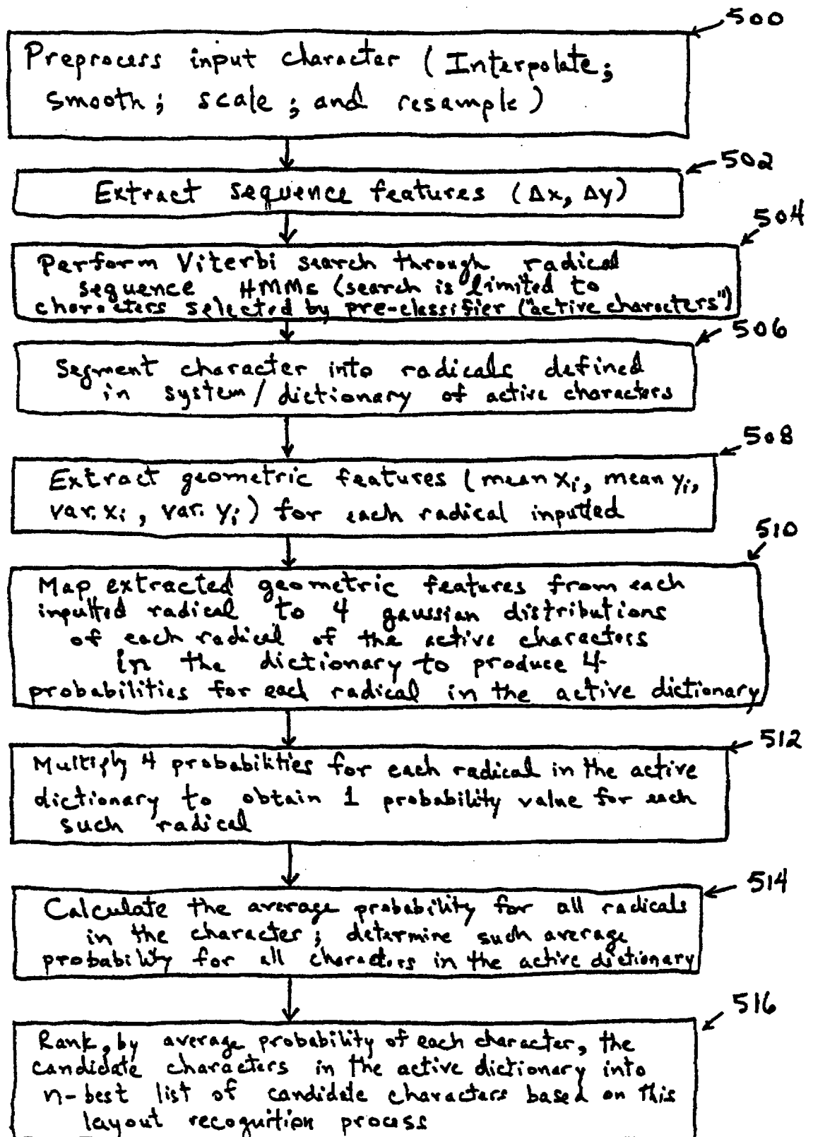
Figure 18 - Geometric Layout Recognition
