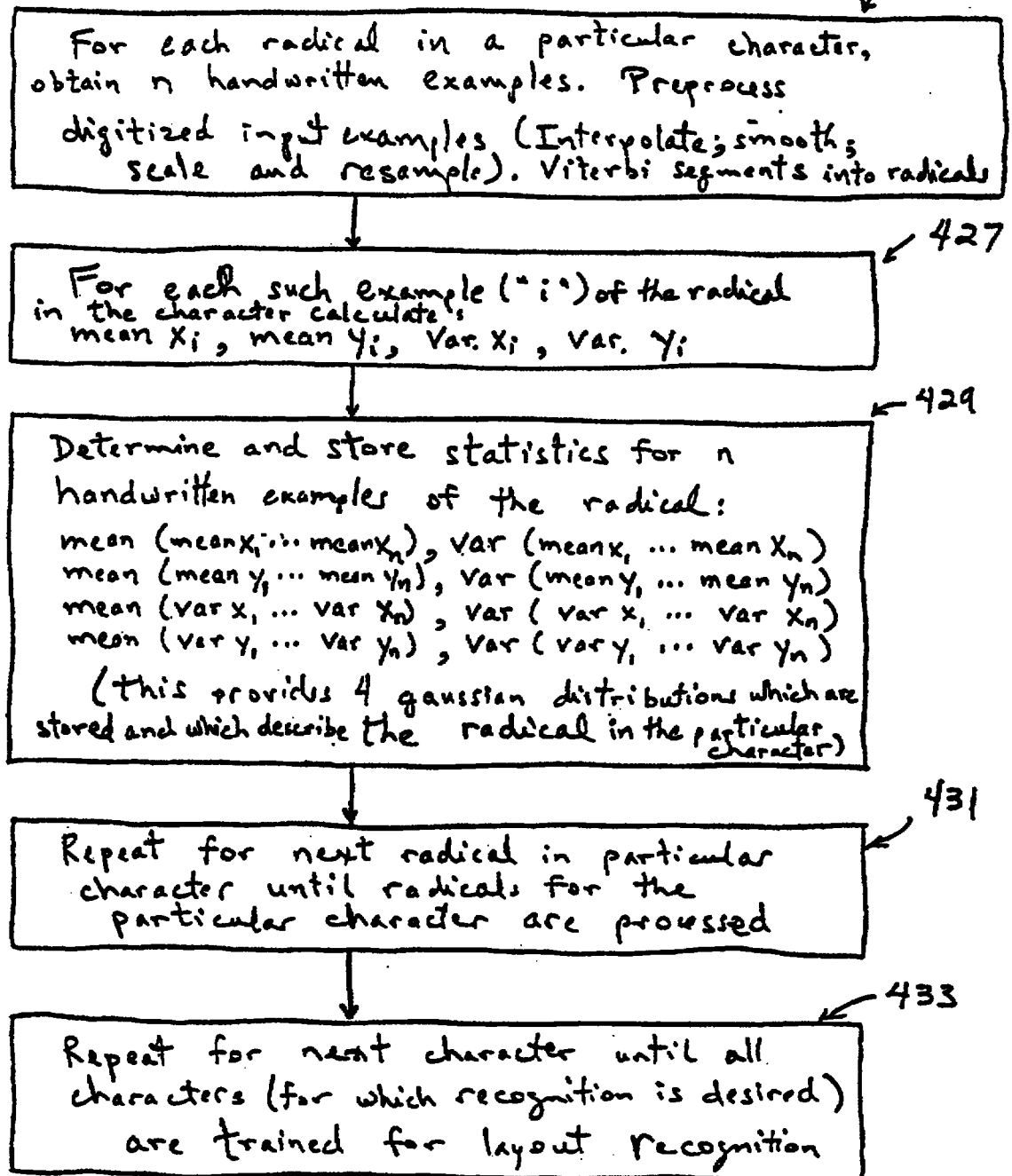
Figure 16 - Geometric Layout Training
