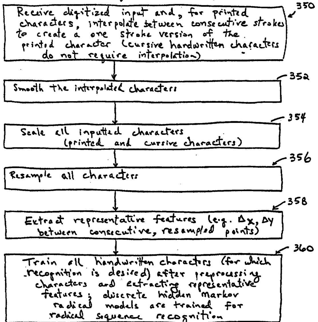
Figure 11 - Radical Sequence Training
