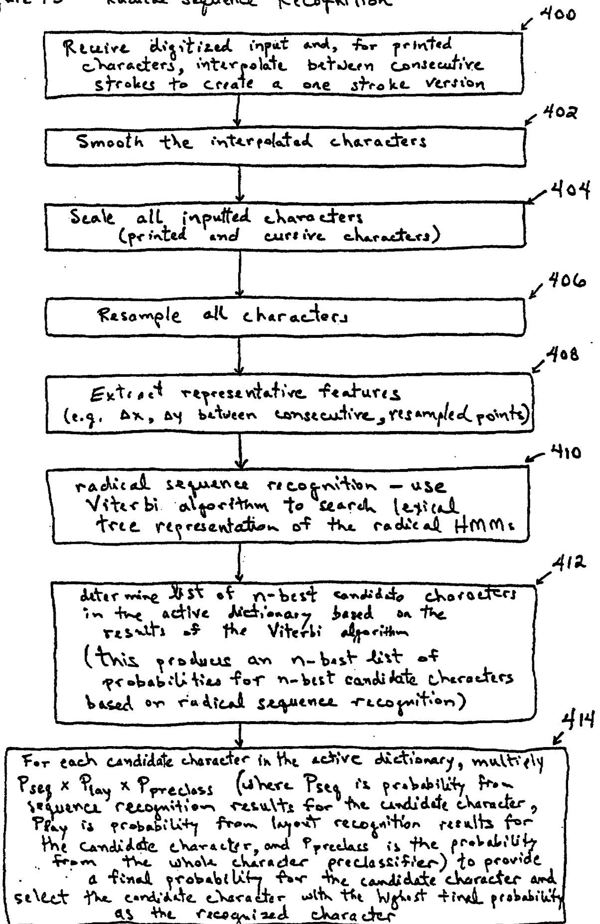
Figure 15 - Radical Sequence Recognition
