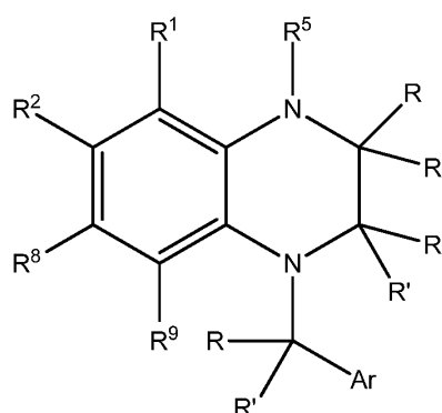
Formula XVI
