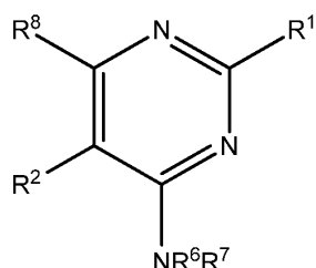
Formula IXa
