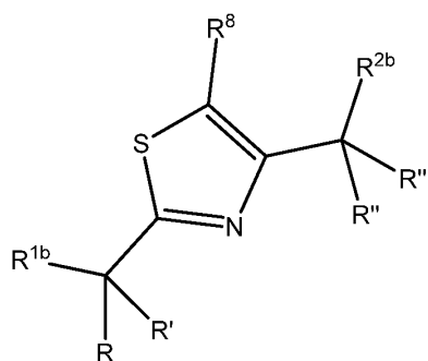
Formula IIIb
