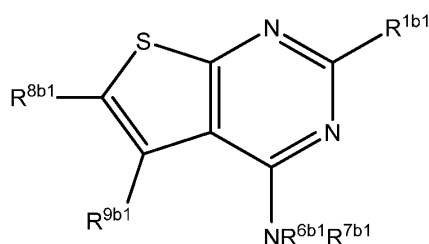
Formula VIIIb1
