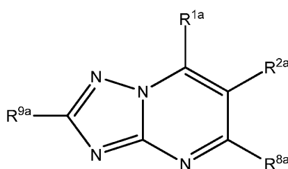
Formula XIIa
