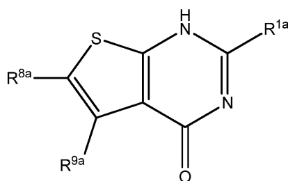
Formula VIa
