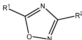
Formula XX
