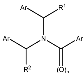
Formula XXIIa
