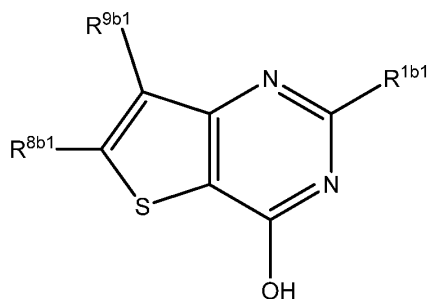
Formula VIb1
