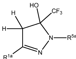
Formula XVa1
