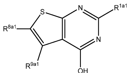
Formula VIa1
