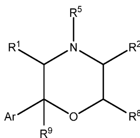
Formula XXI
