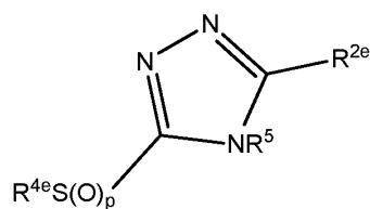
Formula Ie
