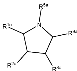
Formula XIXa
