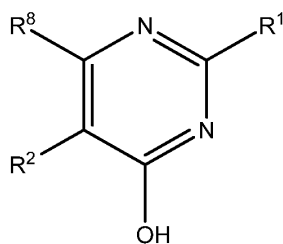
Formula VII
