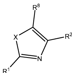
Formula III
