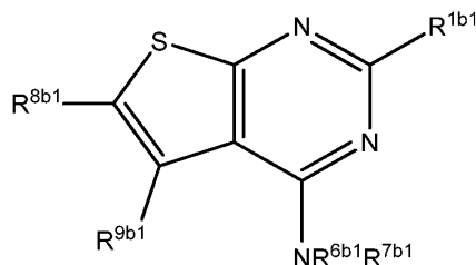
Formula VIIIb1
