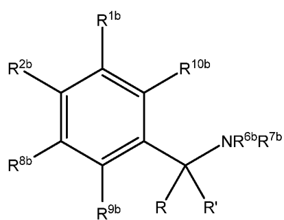
Formula XVIIIb
