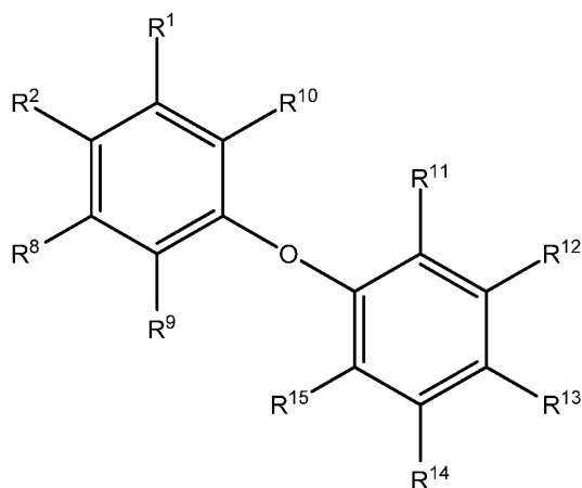
Formula XVII
