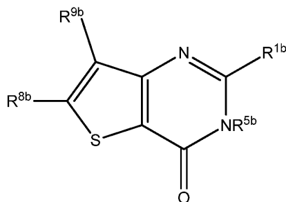
Formula VIb
