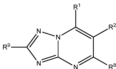
Formula XII
