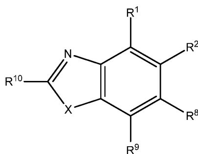
Formula XIV
