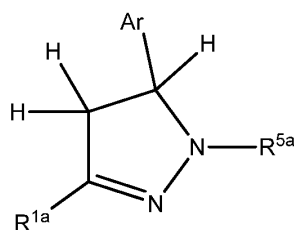
Formula XVb1
