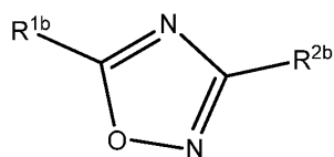
Formula XXb
