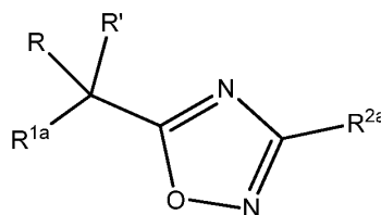
Formula XXa
