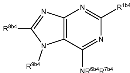
Formula VIIIb4
