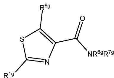
Formula IIIg
