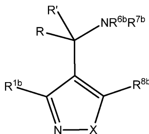
Formula IVb
