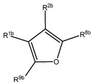
Formula Vb
