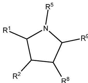
Formula XIX
