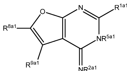
Formula VIIIa1
