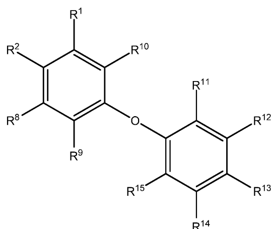
Formula XVII
