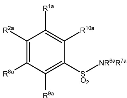
Formula XVIIIa
