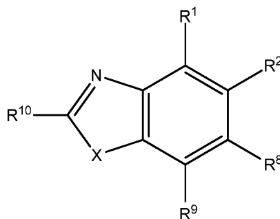
Formula XIV
