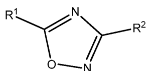
Formula XX
