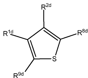
Formula Vd
