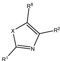
Formula III
