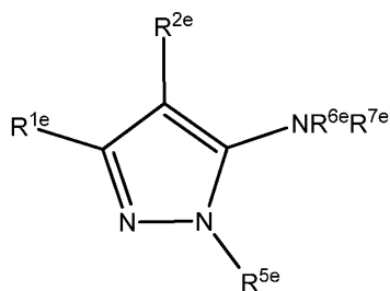
Formula IVe
