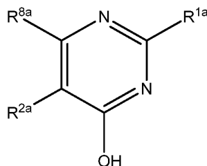
Formula VIIa
