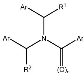
Formula XXII
