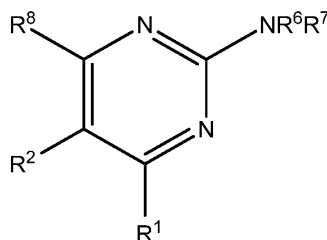
Formula X 456
