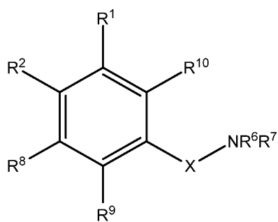
Formula XVIII
