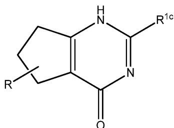
Formula VIc
