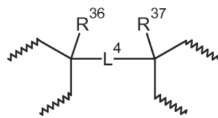
Structure V^b
