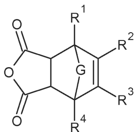
Structure IX
