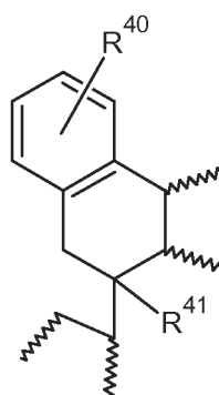
Structure V^h
