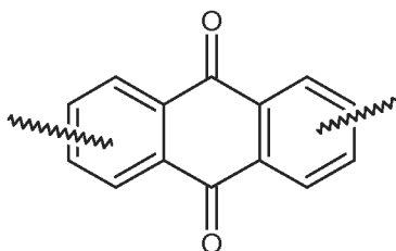
Structure IV b
