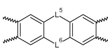
Structure V^c
