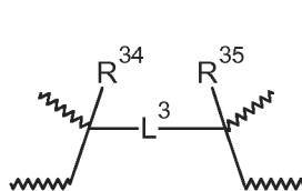
Structure V^a
