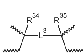
Structure V d
