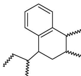
Structure V^b
