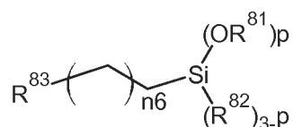
Structure XIV
