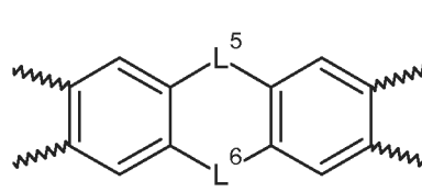
Structure V f
