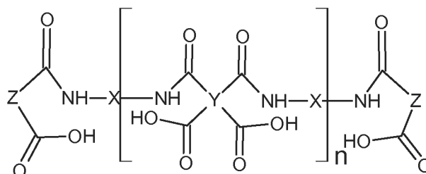
Structure VIII
