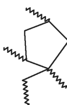
Structure V i
