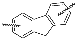
Structure IV a
