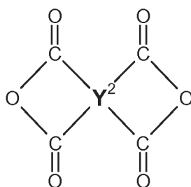
Structure VI
