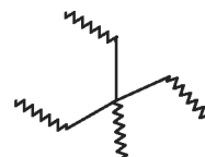
Structure V j
