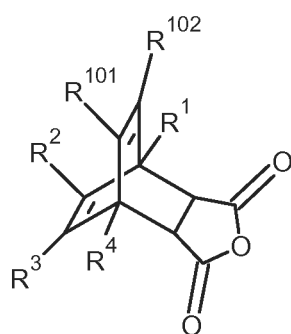
IX c
