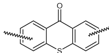
Structure IV c
