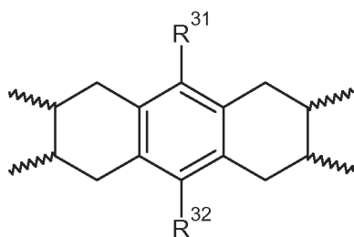
Structure V a
