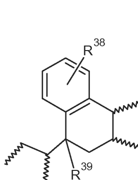
Structure V^g
