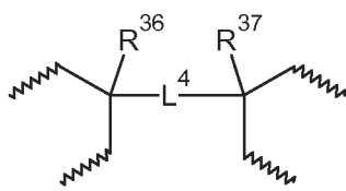
Structure V e
