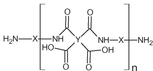
Structure VII
