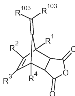
IX d
