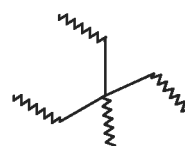
Structure V^j , and
