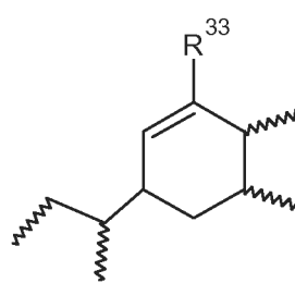
Structure V c
