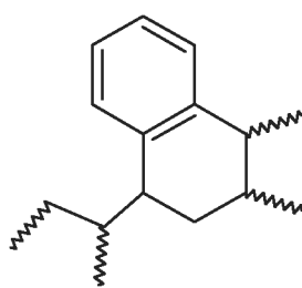
Structure V b
