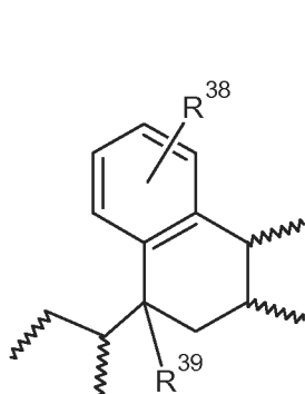
Structure V g
