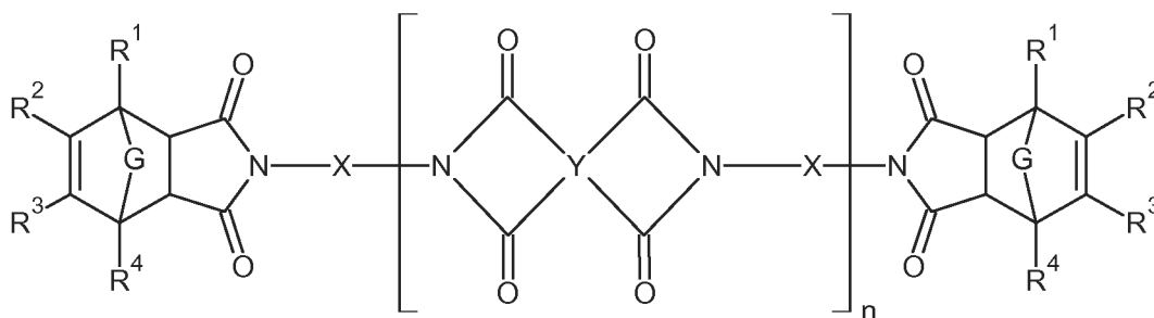
Structure II
