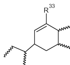
Structure V^c
