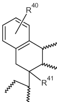
Structure V h
