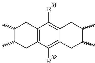
Structure V^a
