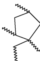
Structure V^i
