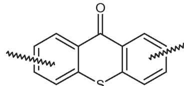
Structure IV c
