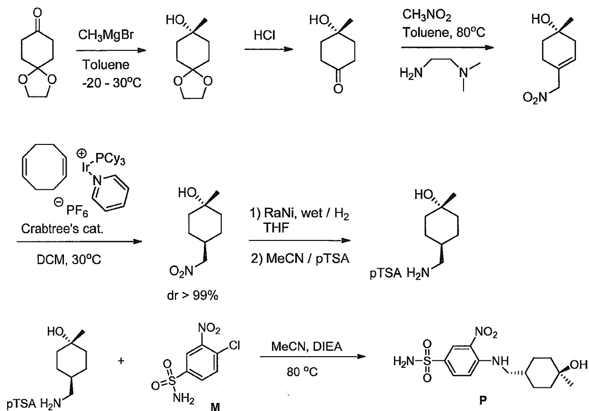
Scheme 4'
