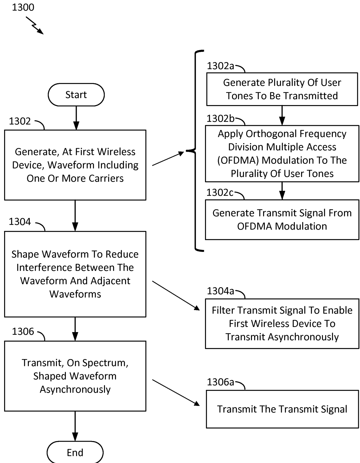
FIG. 13 OFDMA with WOLA (OFDMA Transmitter)
