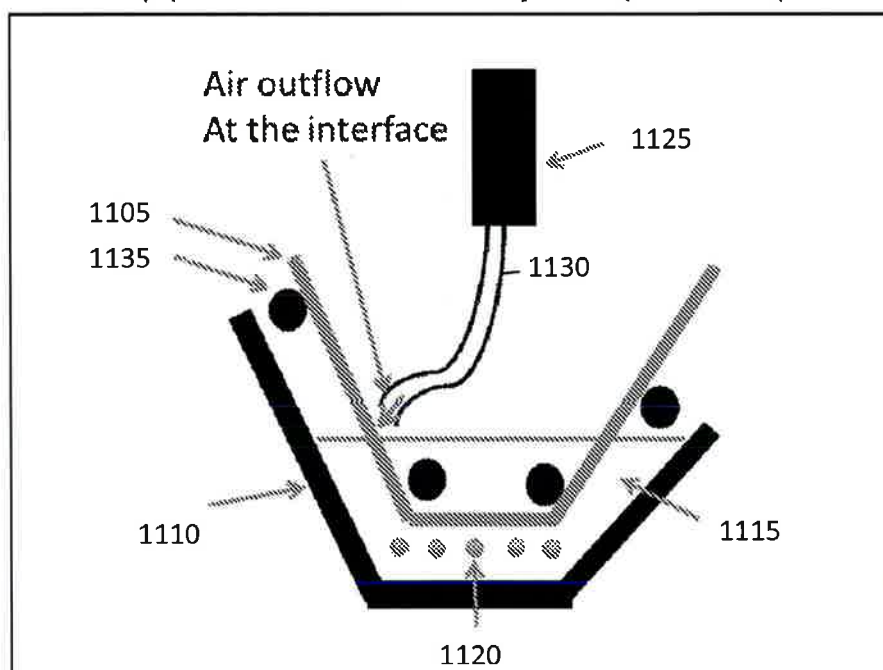
(a) Solution Treatment System (side view)
