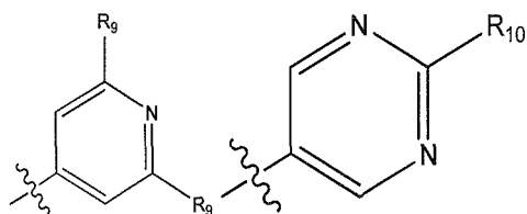
IId
