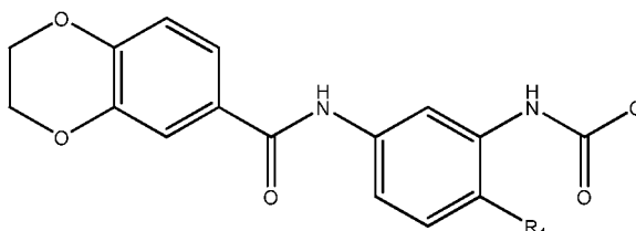
IB
