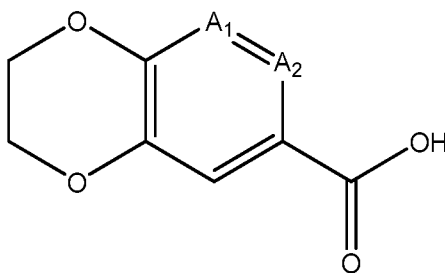
Formula D
