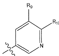
IIc
