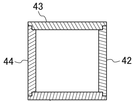
FIG. 10D A-A CROSS-SECTIONAL VIEW
