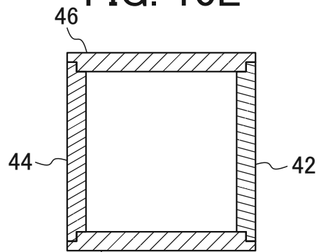
FIG. 10F C-C CROSS-SECTIONAL VIEW
