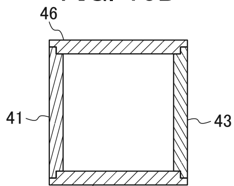
FIG. 10E B-B CROSS-SECTIONAL VIEW
