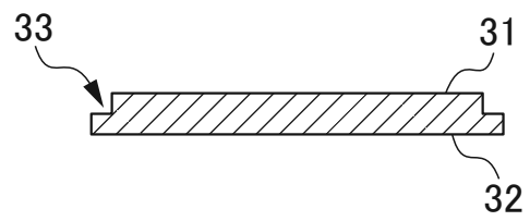
A-A CROSS-SECTIONAL VIEW FIG. 4C
