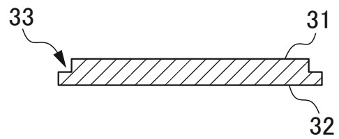
B-B CROSS-SECTIONAL VIEW FIG. 4D
