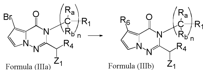
Scheme 7
