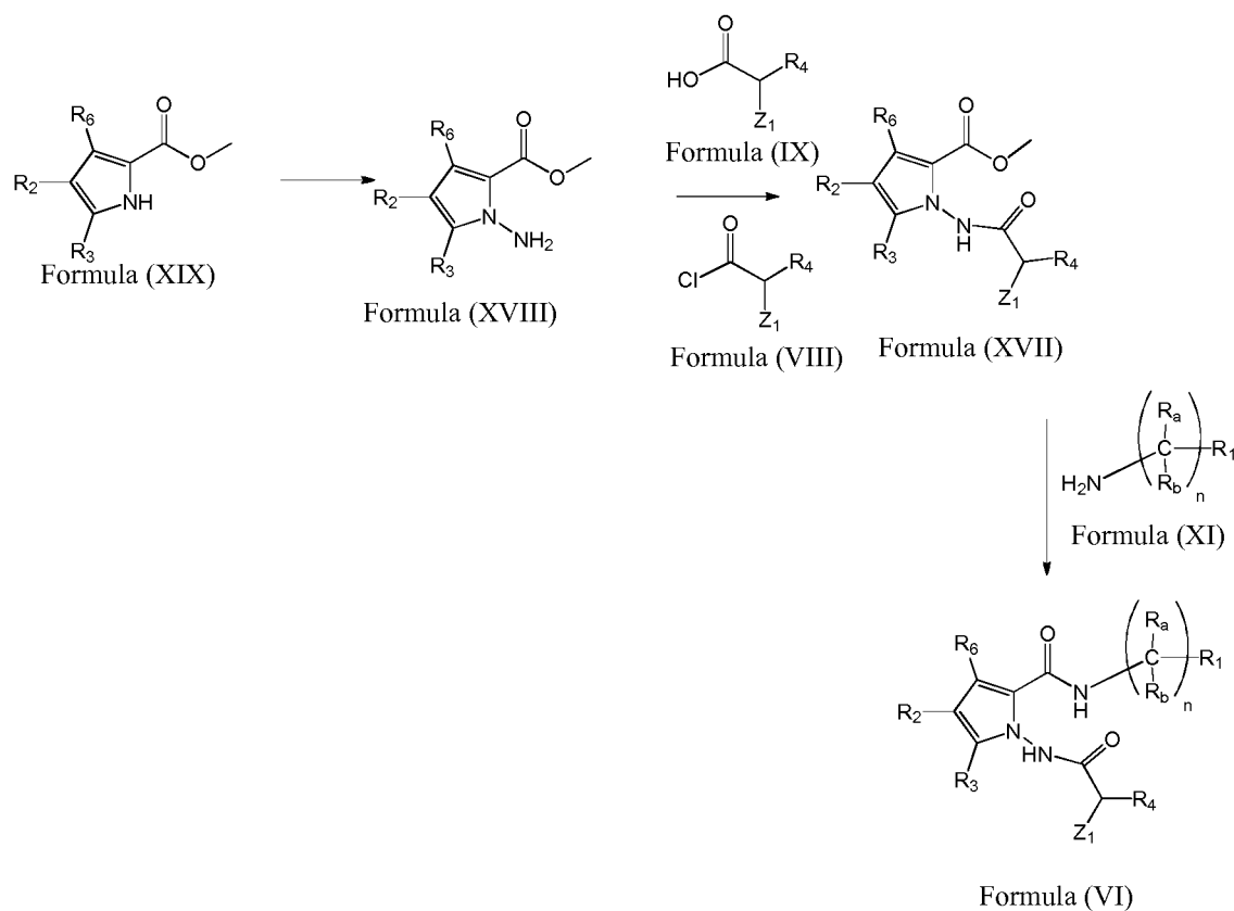
Scheme 6
