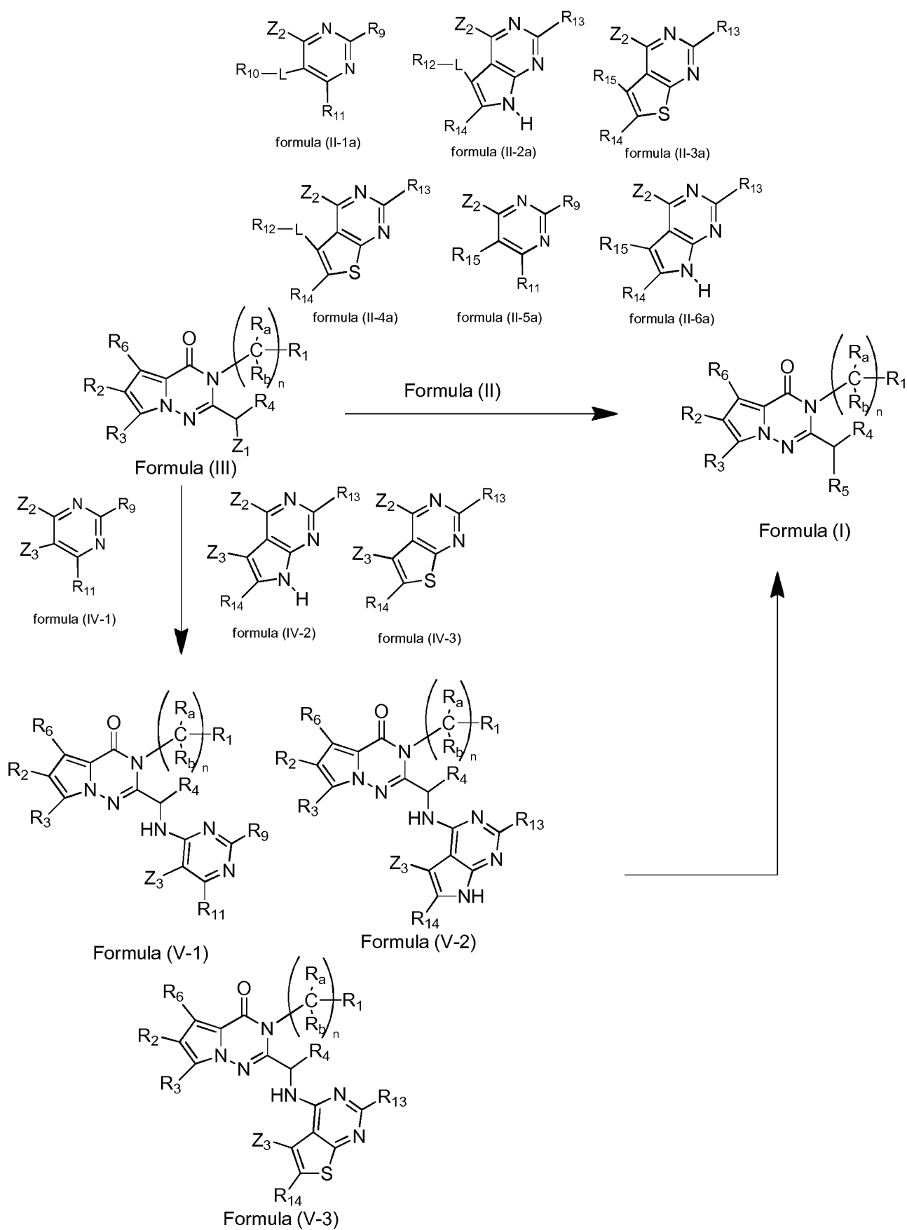
Scheme 1
