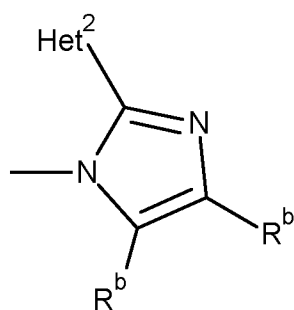
Het1/2f
