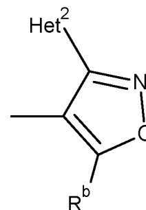
Het1/2c
