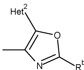
Het1/2b
