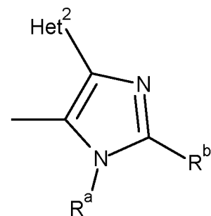
Het1/2h
