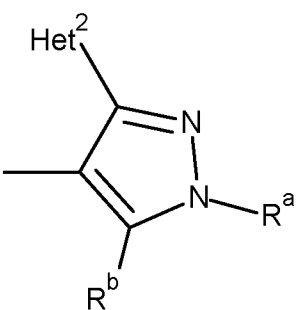
Het1/2d
