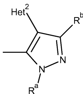
Het1/2q
