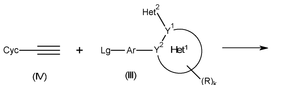
10 Scheme 3:
