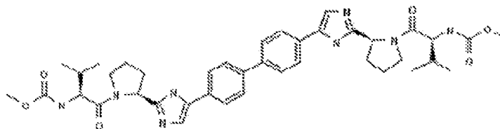
Daclatasvir dihydrochloride
