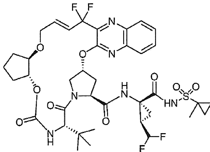
Compound 1
