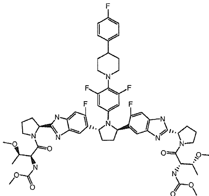
Compound 2
