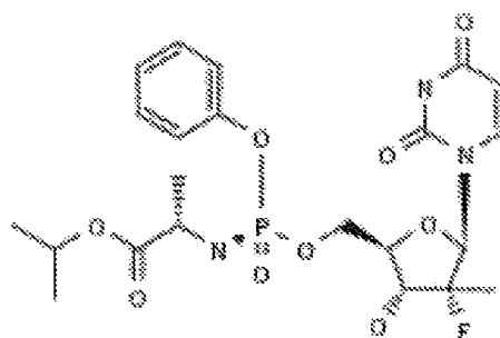
PSI-7977
