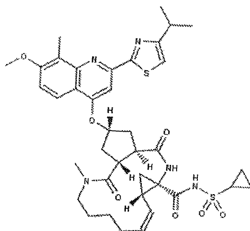
TMC-435 (TMC-435350)
