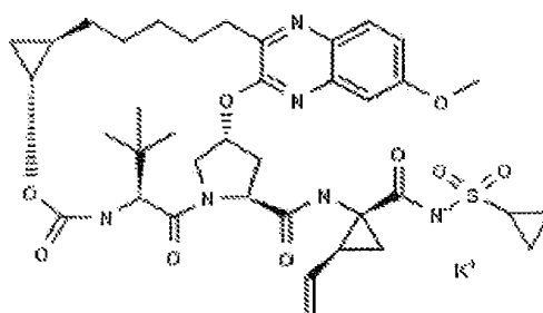
MK-5172
