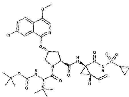
BMS-650032 (Asunaprevir)
