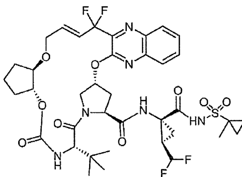
Compound 1
