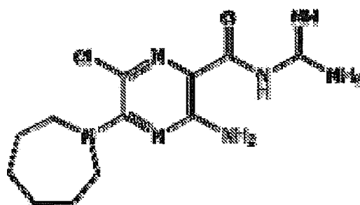
BIT-225
