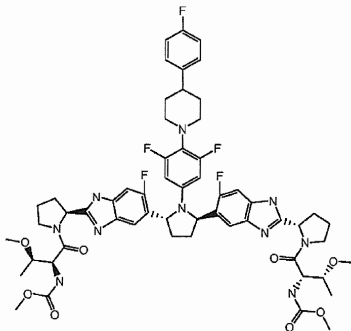
Compound 2
