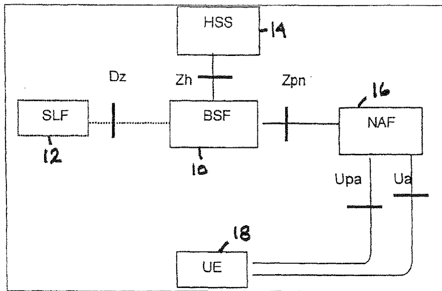
GBA Push architecture FIGURE 1
