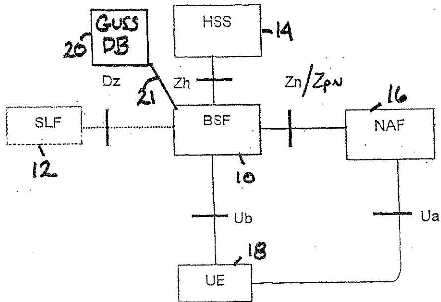
GBA Architecture FIGURE 3
