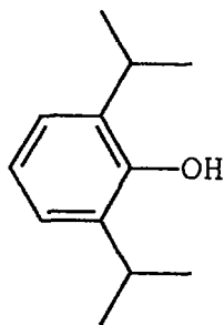
Propofol (2,6-diisopropylphenol)
