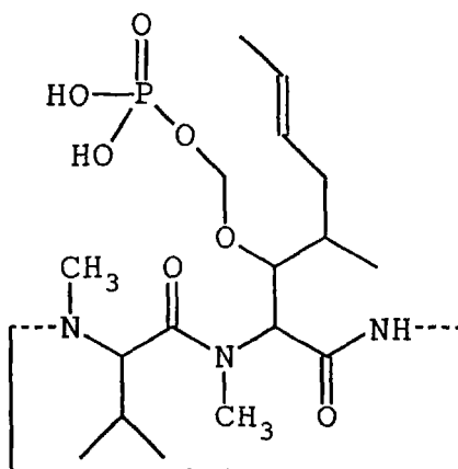
Cyclosporin A
