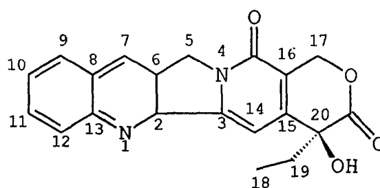
Figure 1 - Camptothecin
