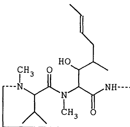
Cyclosporin A
