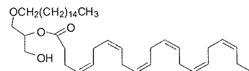
(4Z,7Z,10Z,13Z,16Z,19Z)-1-(hexadecyloxy)-3-hydroxypropan-2-yl docosa-4,7,10,13,16,19-hexaenoate
