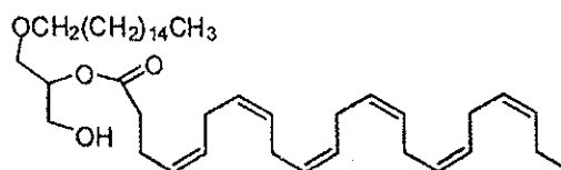
(4Z,7Z,10Z,13Z,16Z,19Z)-1-(hexadecyloxy)-3-hydroxypropan-2-yl docosa-4,7,10,13,16,19-hexaenoate
