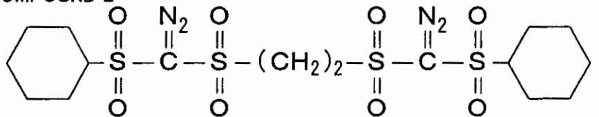
COMPOUND F
