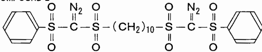
COMPOUND E
