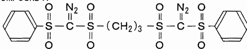
COMPOUND B
