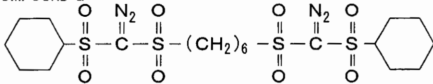
COMPOUND H
