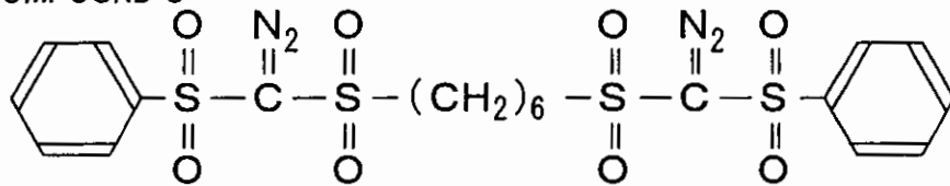
COMPOUND D
