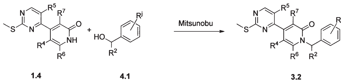
Scheme 4
