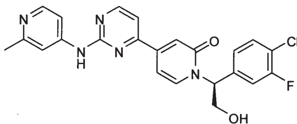
(S)-1-(1-(4-chloro-3-fluorophenyl)-2-hydroxyethyl)-4-(2-((2-methylpyridin-4-yl)amino)pyrimidin-4-yl)pyridin-2(1H)-one
