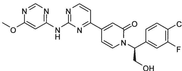
(S)-1-(1-(4-chloro-3-fluorophenyl)-2-hydroxyethyl)-4-(2-((6-methoxypyrimidin-4-yl)amino)pyrimidin-4-yl)pyridin-2(1H)-one
