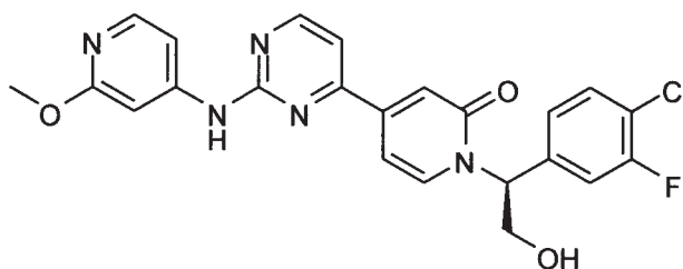
( S )-1-(1-(4-chloro-3-fluorophenyl)-2-hydroxyethyl)-4-(2-((2-methoxypyridin-4-yl)amino)pyrimidin-4-yl)pyridin-2(1 H )-one
