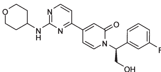
( S )-1-(1-(3-fluorophenyl)-2-hydroxyethyl)-4-(2-((tetrahydro-2 H -pyran-4-yl)amino)pyrimidin-4-yl)pyridin-2(1 H )-one
