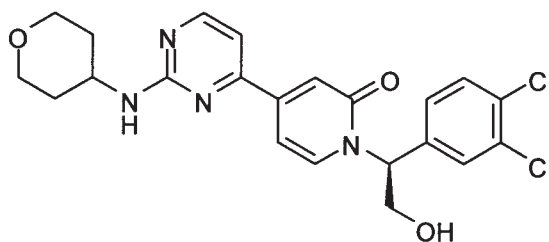
( S )-1-(1-(3,4-dichlorophenyl)-2-hydroxyethyl)-4-(2-((tetrahydro-2 H -pyran-4-yl)amino)pyrimidin-4-yl)pyridin-2(1 H )-one
