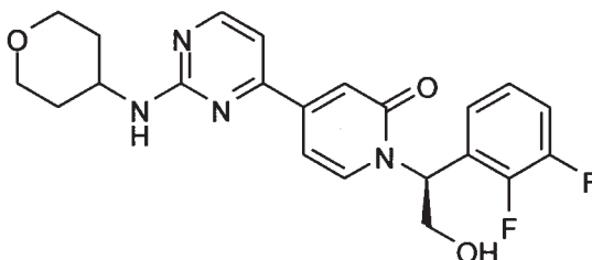
( S )-1-(1-(2,3-difluorophenyl)-2-hydroxyethyl)-4-(2-((tetrahydro-2 H -pyran-4-yl)amino)pyrimidin-4-yl)pyridin-2(1 H )-one
