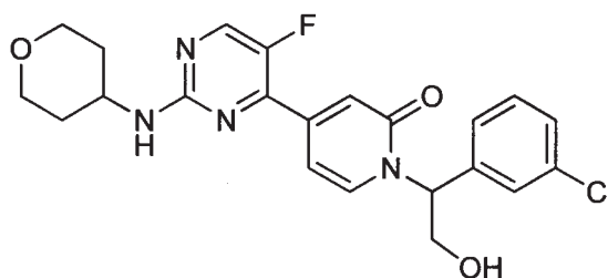
1-(1-(3-chlorophenyl)-2-hydroxyethyl)-4-(5-fluoro-2-((tetrahydro-2 H -pyran-4-yl)amino)pyrimidin-4-yl)pyridin-2(1 H )-one
