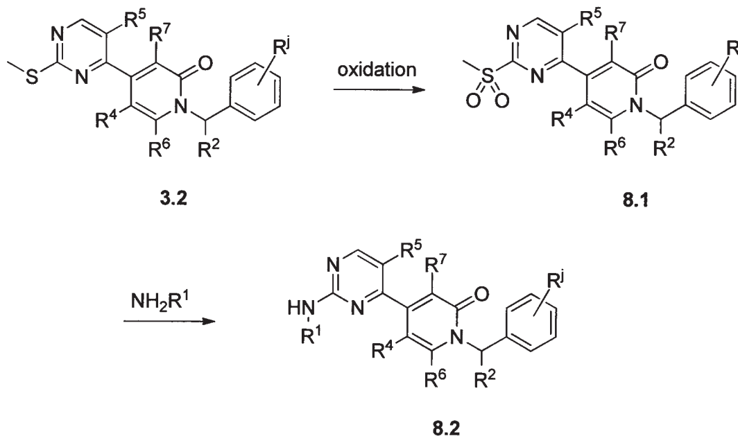
Scheme 8
