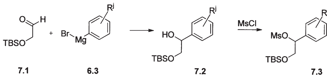
Scheme 7
