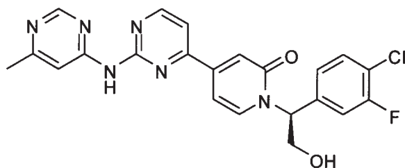
(S)-1-(1-(4-chloro-3-fluorophenyl)-2-hydroxyethyl)-4-(2-((6-methylpyrimidin-4-yl)amino)pyrimidin-4-yl)pyridin-2(1H)-one
