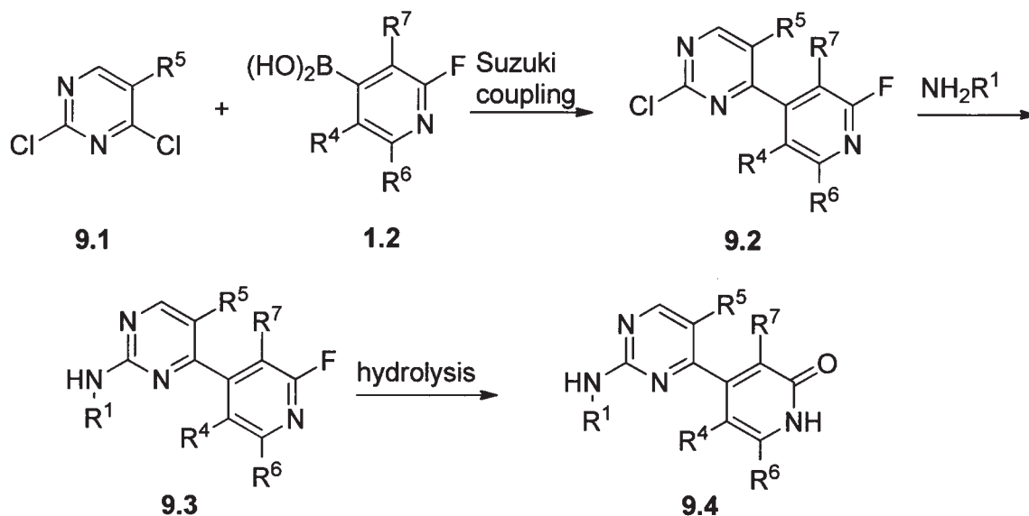
Scheme 9
