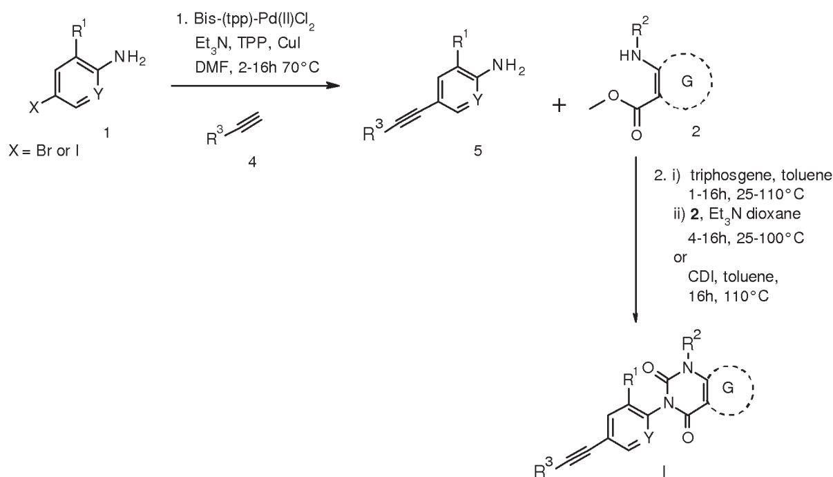
Scheme 2
