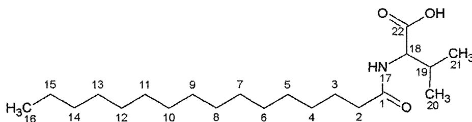
Structure 65 Val-C16:0
