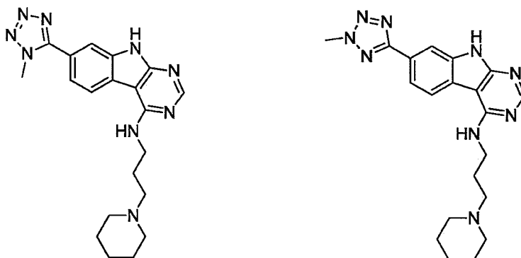
7-(1-methyl-1H-tetrazol-5-yl)-N-(3-(piperidin-1-yl)propyl)-9H-pyrimido[4,5-b]indol-4-amine and 7-(2-methyl-2H-tetrazol-5-yl)-N-(3-(piperidin-1-yl)propyl)-9H-pyrimido[4,5-b]indol-4-amine
