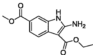
3-ethyl 6-methyl 2-amino-1 H -indole-3,6-dicarboxylate
