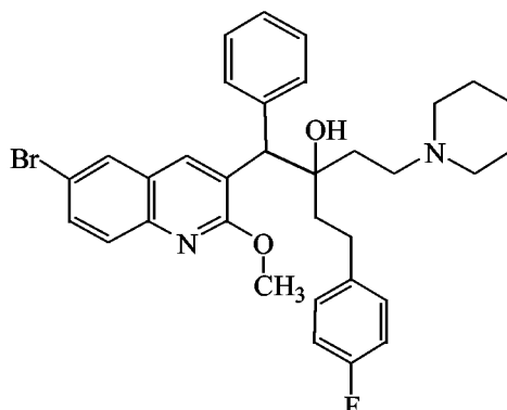
Compound 35 (dia B)
