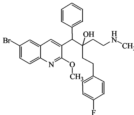
Compound 40 (dia B)
