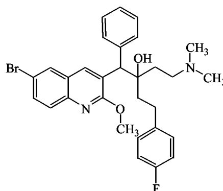
Compound 28 (B2)
