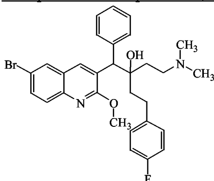
Compound 25 (A1)
