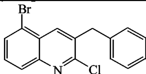
intermediate 6
