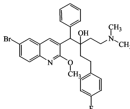
Compound 26 (A2)
