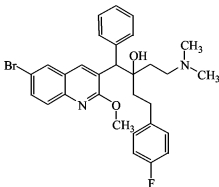
Compound 27 (B1)
