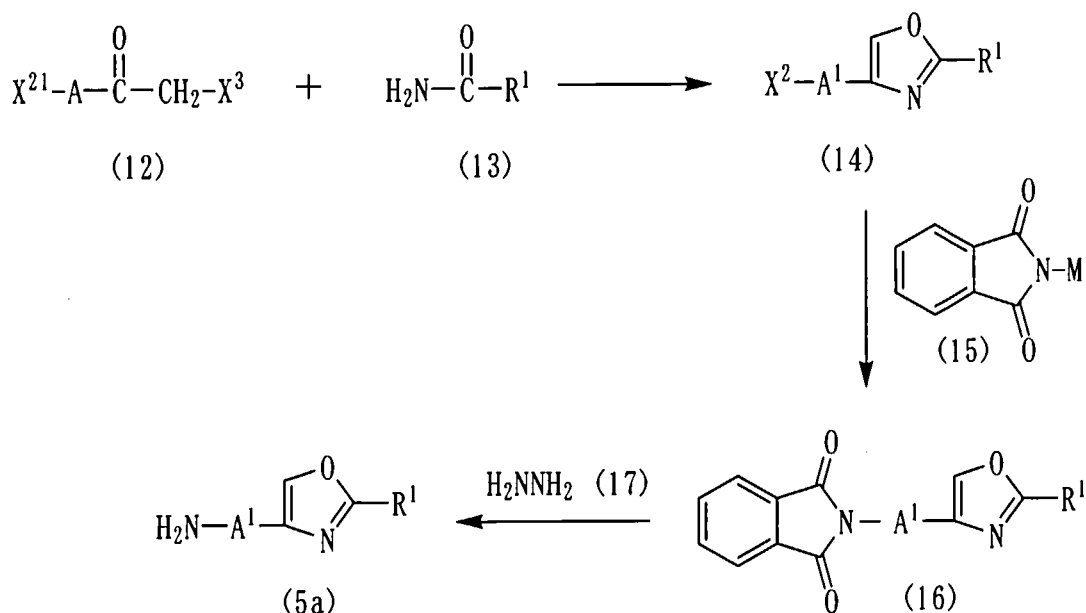
Reaction Scheme 10
