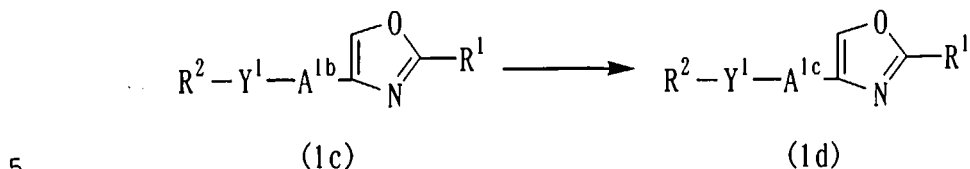
Reaction Scheme 4
