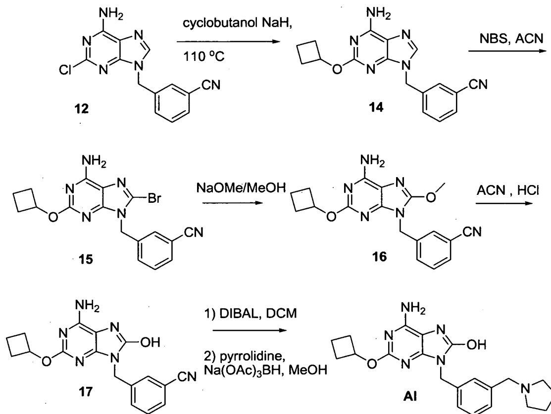
Scheme 12
