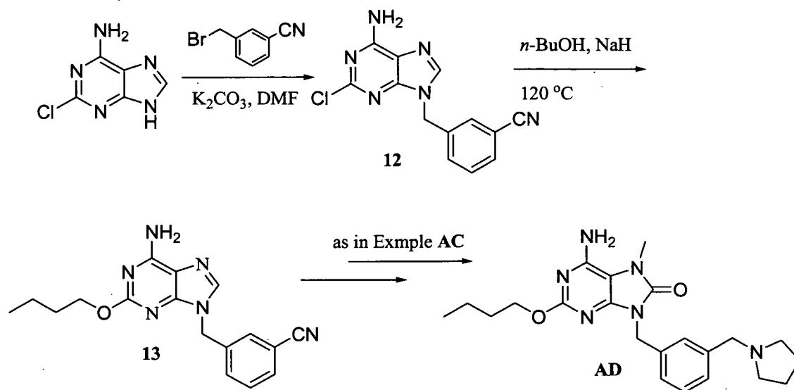
Scheme 11
