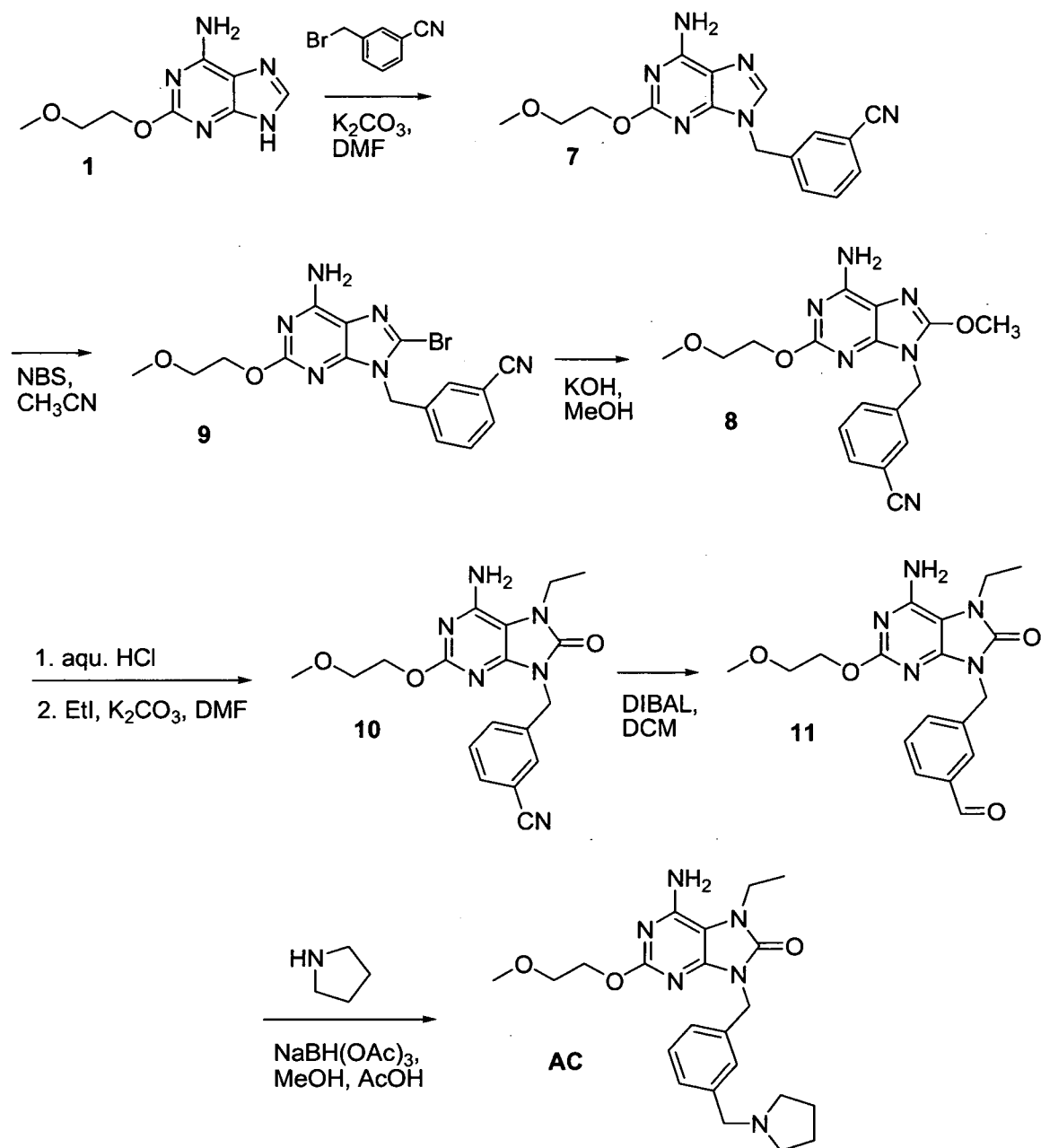
Scheme 10
