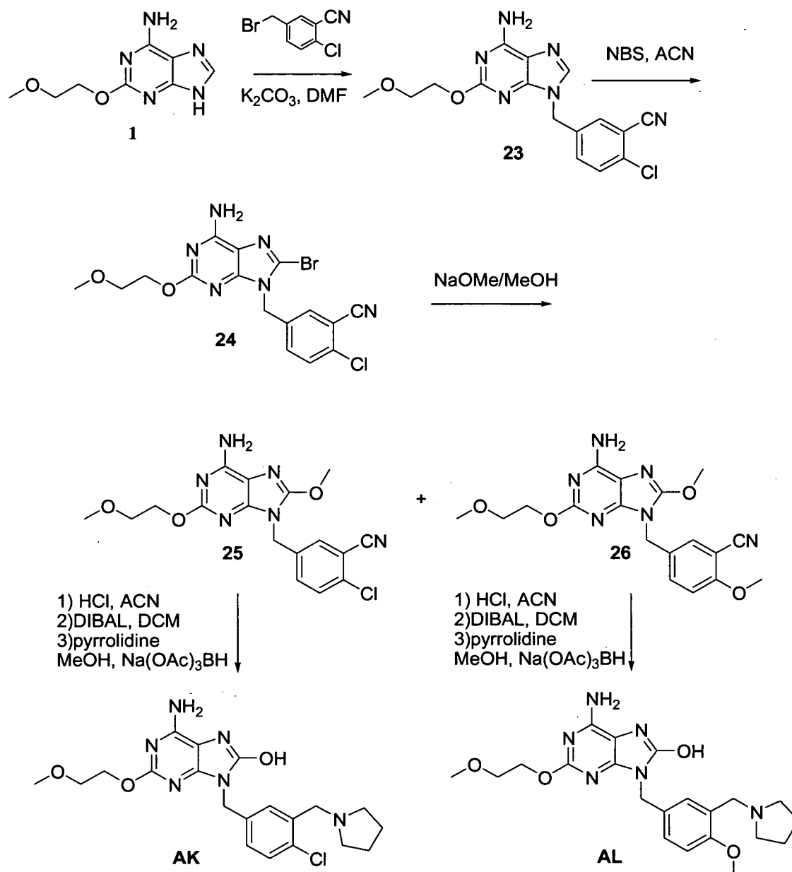
Scheme 14
