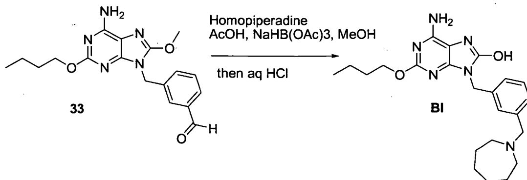
Scheme 19
