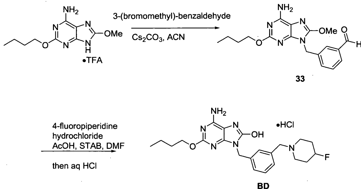
Scheme 17
