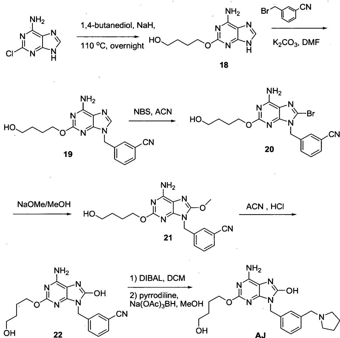
Scheme 13
