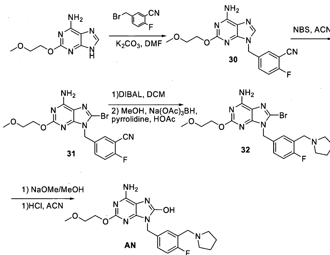
Scheme 16
