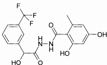
N' -[2-Hydroxy-2-(3-trifluoromethylphenyl)acetyl]-2,4-dihydroxy-6-methylbenzohydrazide
