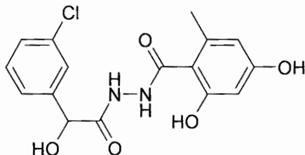
N' -[2-Hydroxy-2-(3-chlorophenyl)acetyl]-2,4-dihydroxy-6-methylbenzohydrazide
