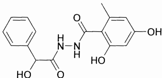
N' -(2-Hydroxy-2-phenylacetyl)-2,4-dihydroxy-6-methylbenzohydrazide
