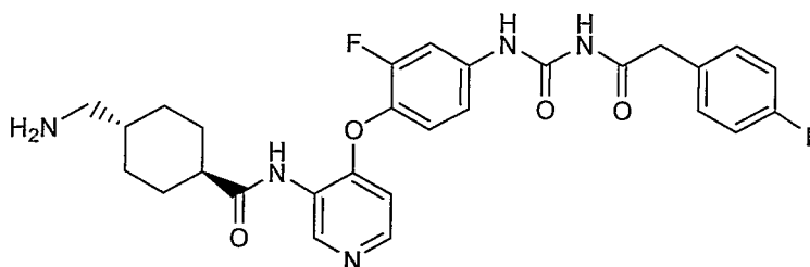
1-(4-(3-((1R,4R)-4-(Aminomethyl)cyclohexanecarboxamido)pyridin-4-yloxy)-3-fluorophenyl)-3-(2-(4-fluorophenyl)acetyl)urea
