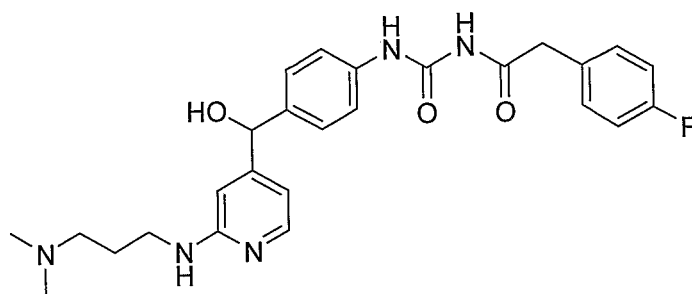
1-(4-((2-(3-(Dimethylamino)propylamino)pyridin-4-yl)(hydroxy)methyl)phenyl)- 3-(2-(4-fluorophenyl)acetyl)urea
