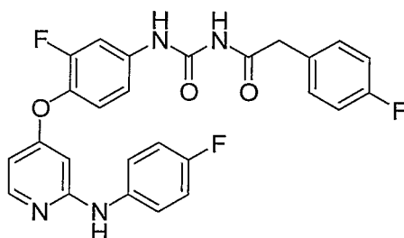
1-(3-Fluoro-4-(2-(4-fluorophenylamino)pyridin-4-yloxy)phenyl)-3-(2-(4-fluorophenyl)acetyl)urea
