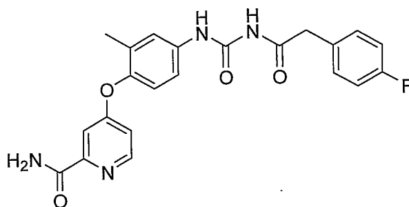
1-(4-(2-Carbamoylpyridin-4-yloxy)-3-methylphenyl)-3-(2-(4-fluorophenyl)acetyl)urea
