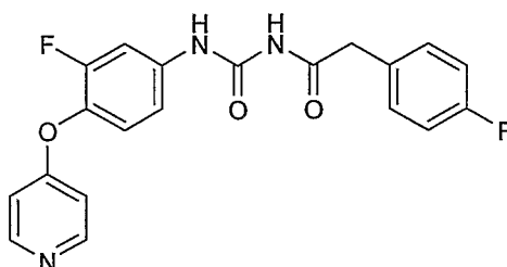
1-(3-Fluoro-4-(pyridin-4-yloxy)phenyl)-3-(2-(4-fluorophenyl)acetyl)urea
