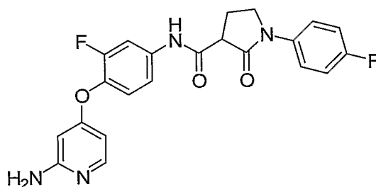
N -(4-(2-Aminopyridin-4-yloxy)-3-fluorophenyl)-1-(4-fluorophenyl)-2-oxopyrrolidine-3-carboxamide
