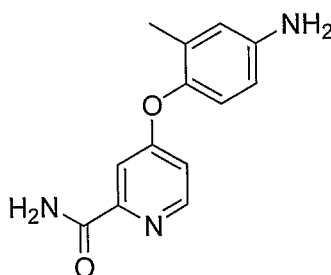
1-(4-(2-Carbamoylpyridin-4-yloxy)-3-methylphenyl)-3-(2-(4-fluorophenyl)acetyl)urea
