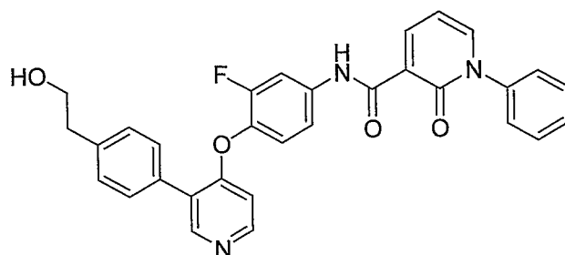
N -(3-Fluoro-4-(3-(4-(2-hydroxyethyl)phenyl)pyridin-4-yloxy)phenyl)-2-oxo-1-phenyl-1,2-dihydropyridine-3-carboxamide
