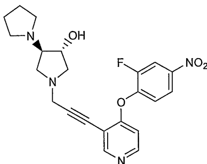
A) (3R,4R)-1-(3-(4-(2-Fluoro-4-nitrophenoxy)pyridin-3-yl)prop-2-ynyl)-4-(pyrrolidin-1-yl)pyrrolidin-3-ol
