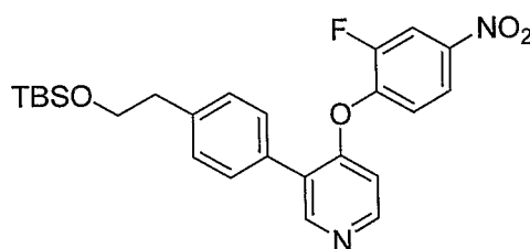
N -(3-Fluoro-4-(3-(4-(2-hydroxyethyl)phenyl)pyridin-4-yloxy)phenyl)-2-oxo-1-phenyl-1,2-dihydropyridine-3-carboxamide
